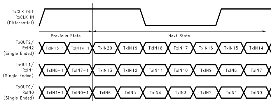
Figure 10. 21 Parallel TTL Data Inputs Mapped to LVDS Outputs
