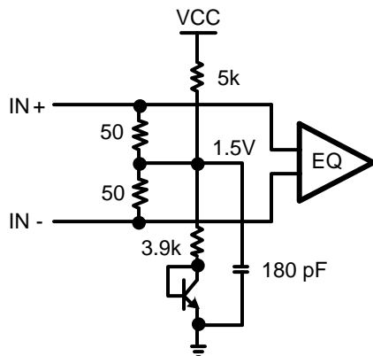
Figure 7. Receiver Input Termination and Bias Circuit
