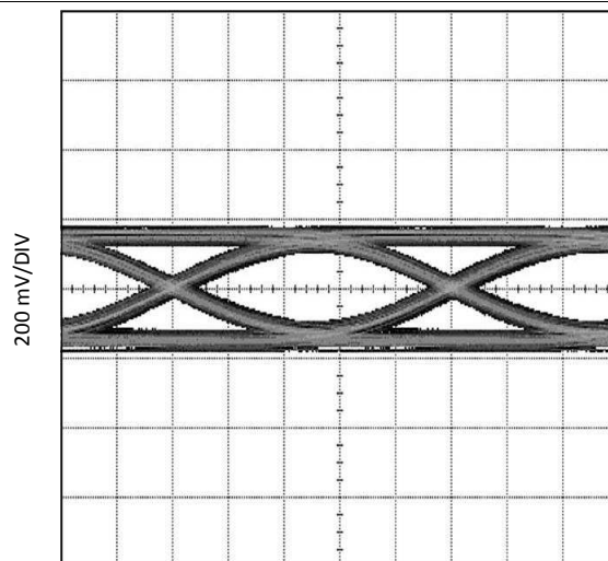
Figure 17. Eye Measured at Point (D), Pre-Emph = -9 dB
