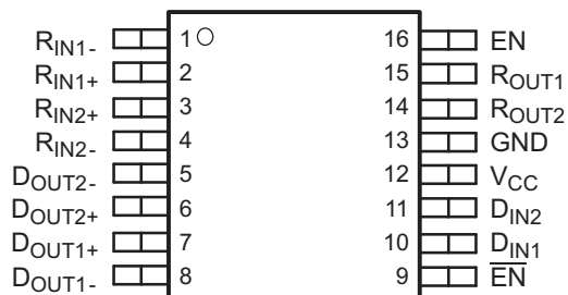
PW Package (Marked as LVDS049) 16-Pin TSSOP (Top View)
