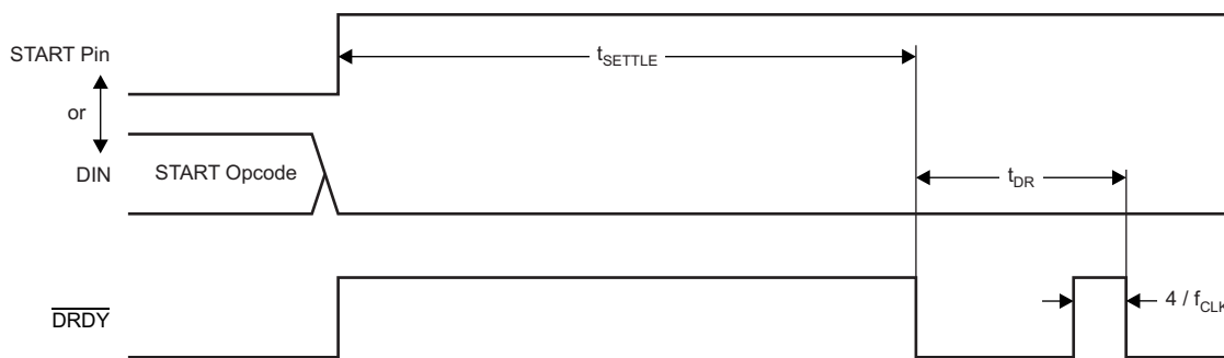
Figure 32. Settling Time
