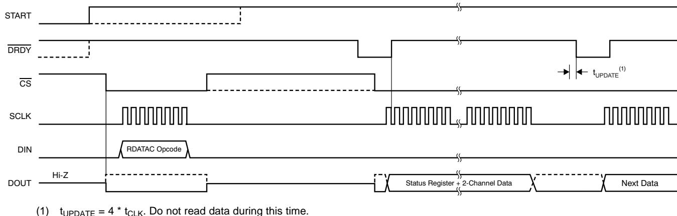
Figure 38. RDATA Usage
