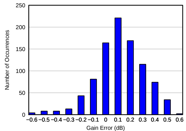
Figure 5. Gain Matching Histogram, V_{CNTL} = 0.6\text{V} (936 Channels)
