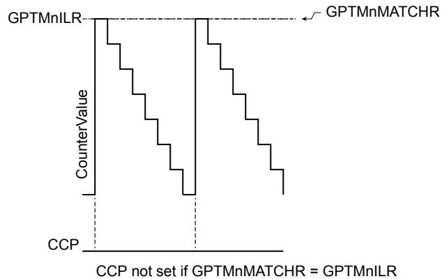
Figure 16-6. CCP Output, GPTMTnMATCHR = GPTMTnILR
