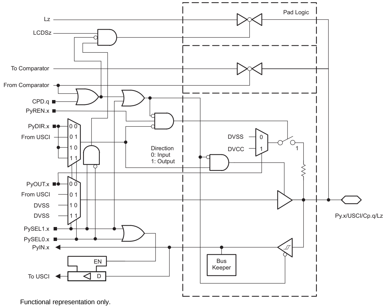
图 6-15. Py.x/USCI/Cp.q Pin Schematic
