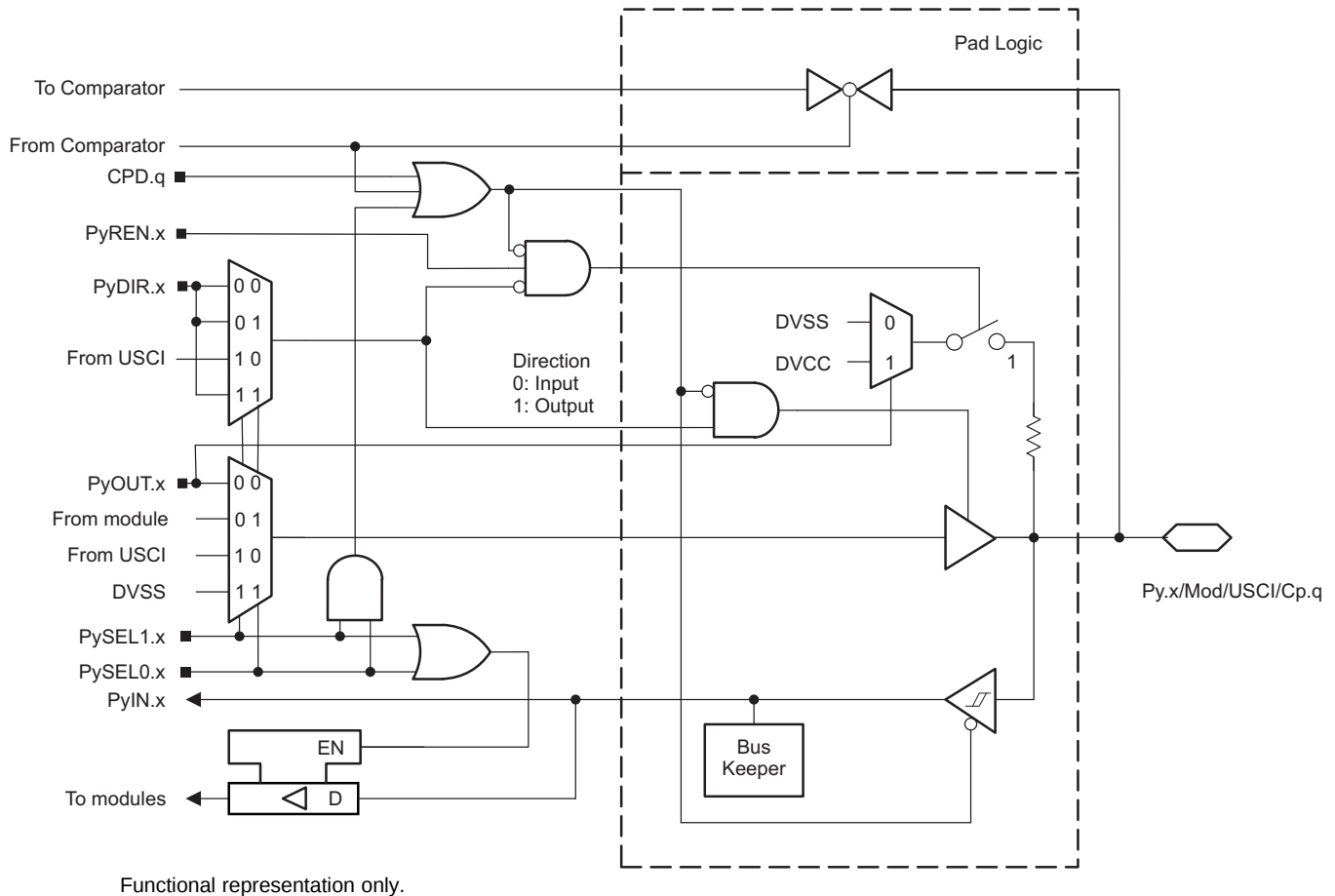
图 6-16. Py.x/Mod/USCI/Cp.q Pin Schematic
