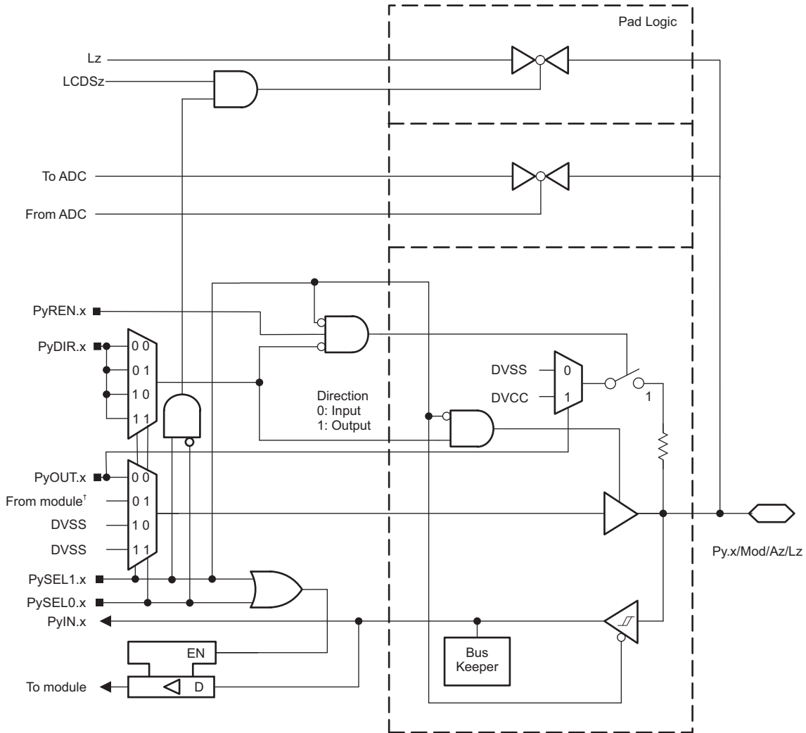
图 6-13. Py.x/Mod/Az/Lz Pin Schematic
