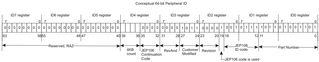
图 6-25. ROM PID Entries for MSP432P4x1xT Device
