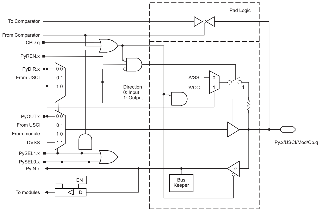
图 6-17. Py.x/USCI/Mod/Cp.q Pin Schematic
