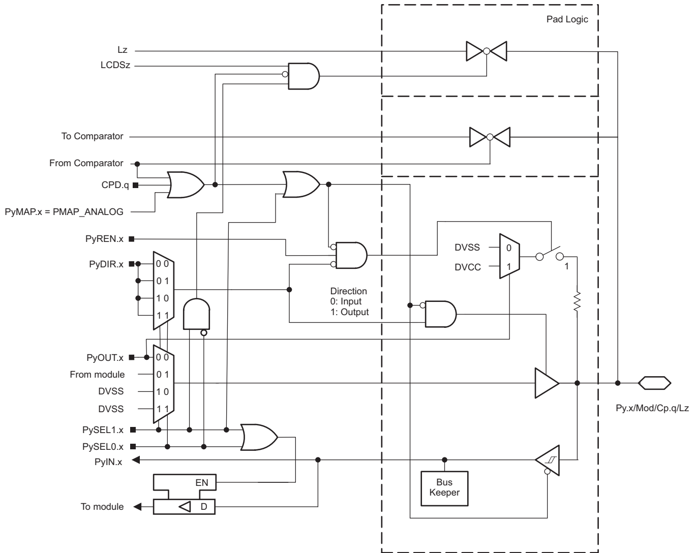
图 6-19. Py.x/Mod/Cp.q/Lz Pin Schematic
