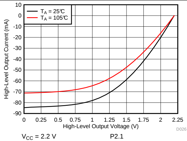
图 5-25. High-Level Output Voltage vs High-Level Output Current
