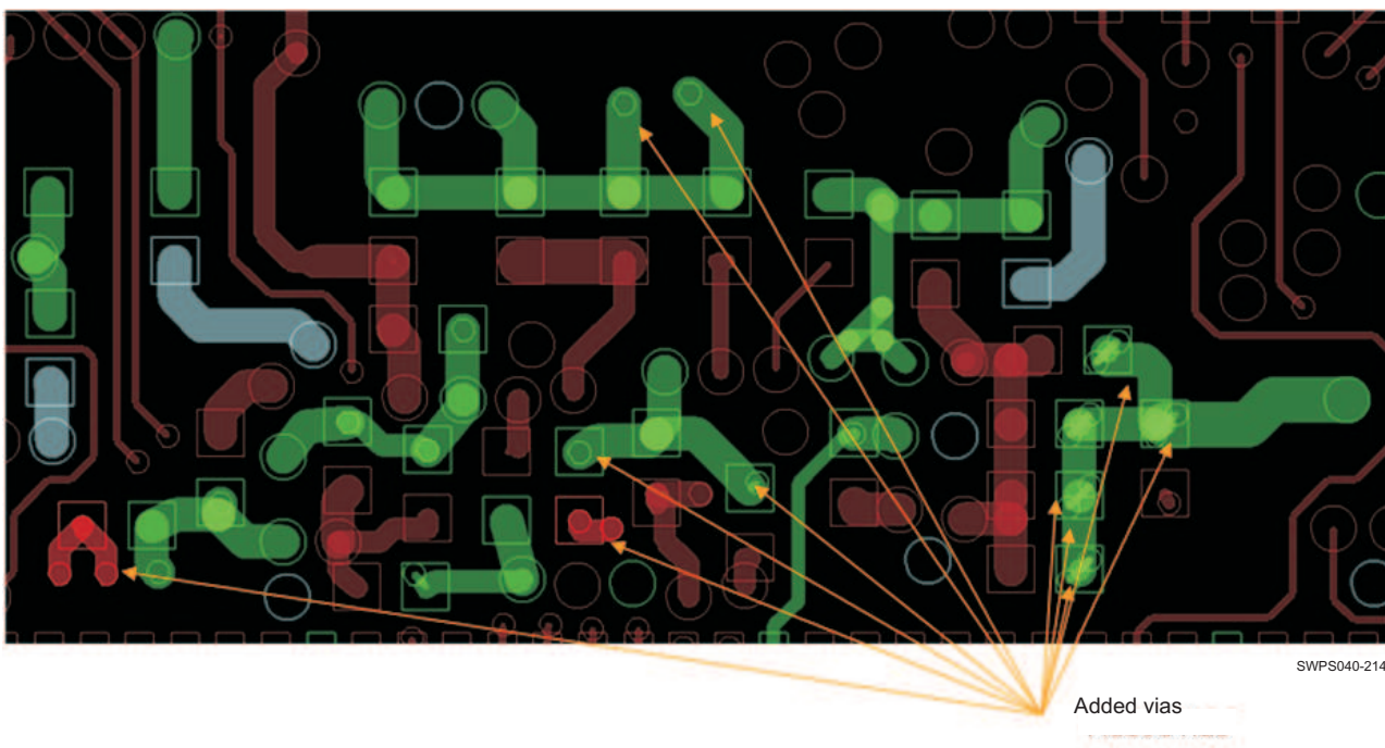
图 7-7. Improved Layout With More Transitional Vias
