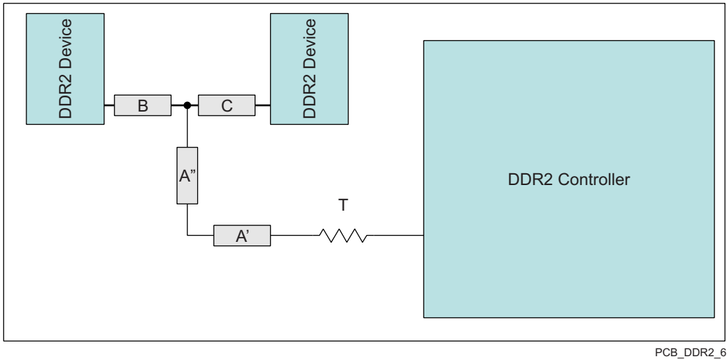
图 7-55. CK and ADDR_CTRL Routing and Topology
