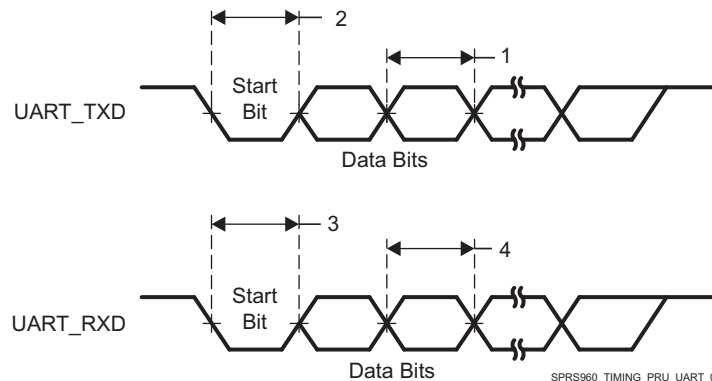
图 5-129. PRU-ICSS UART Timing
