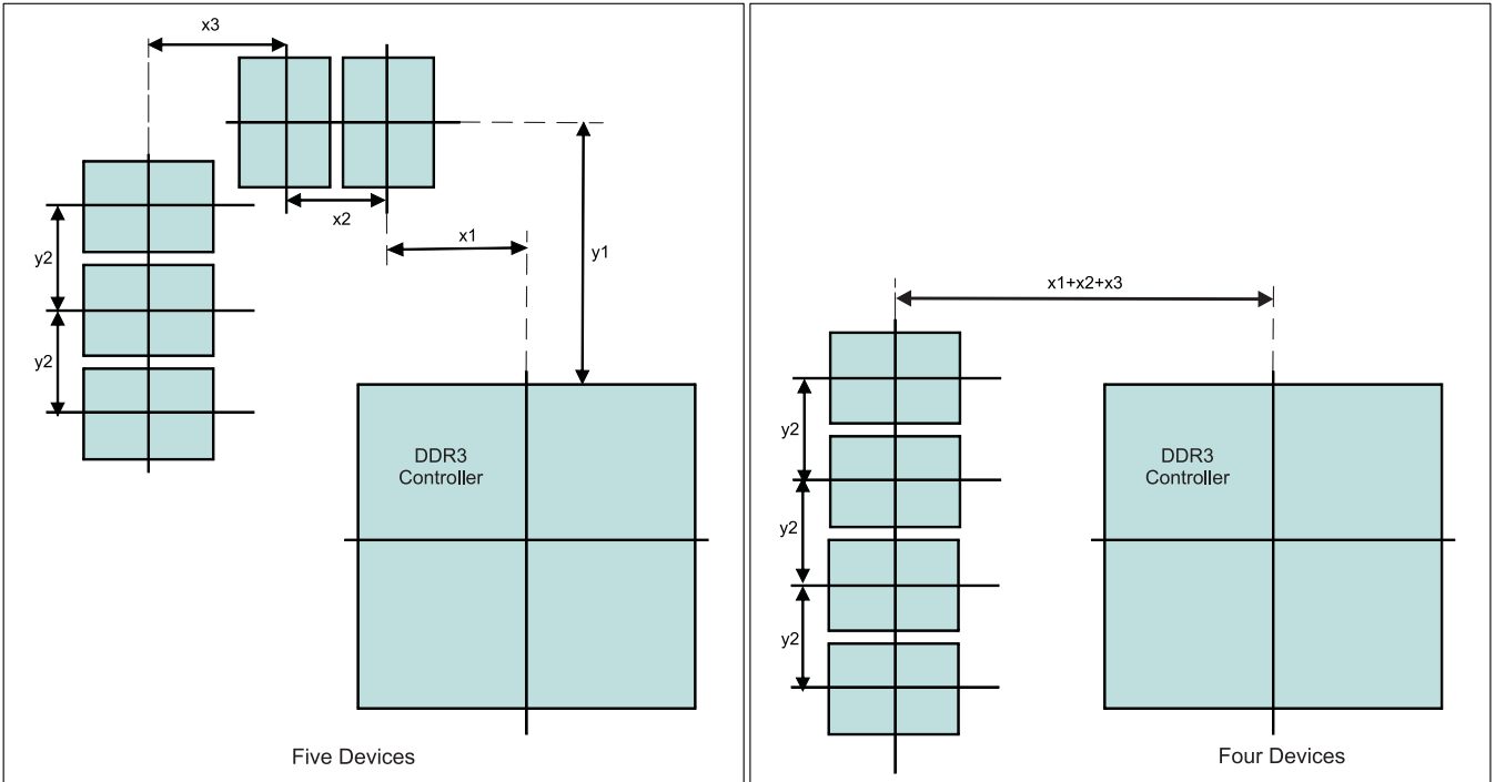
图 7-40. Placement Specifications
