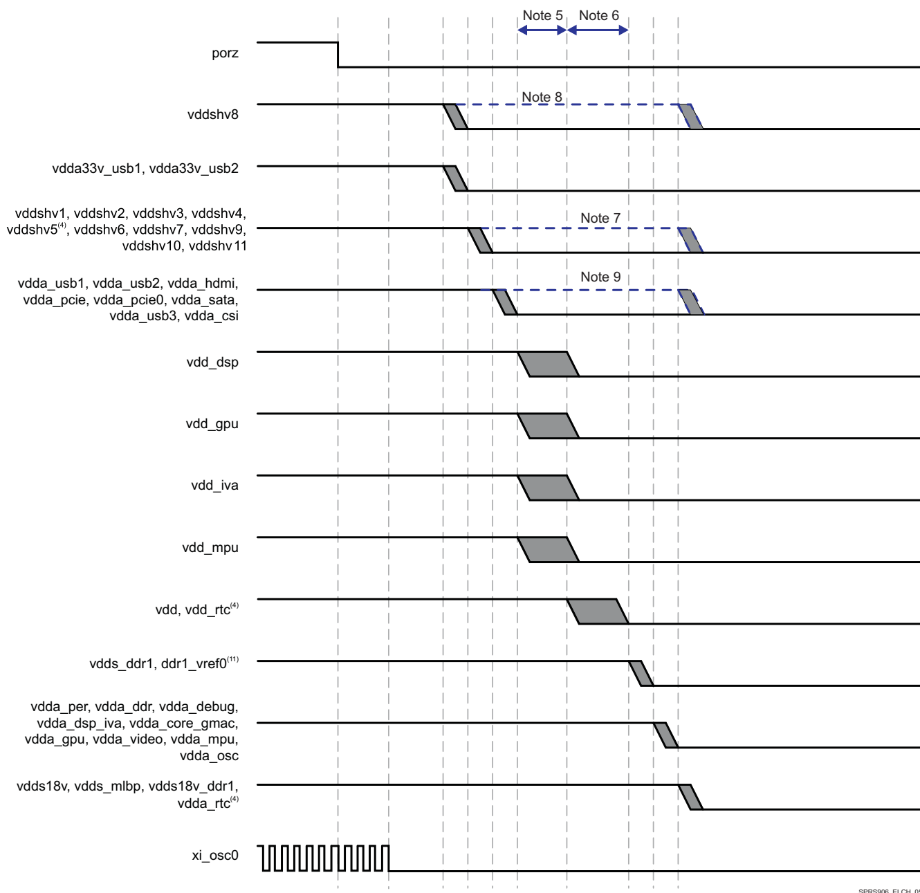
图 5-3. Power-Down Sequencing (10)(12)
