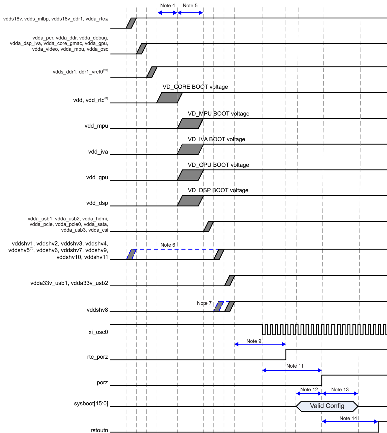
图 5-2. Power-Up Sequencing
