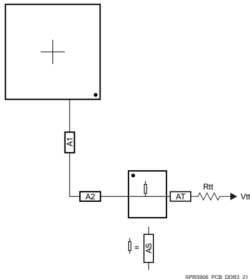
图 8-21. ADDR_CTRL Routing for One DDR3 Device
