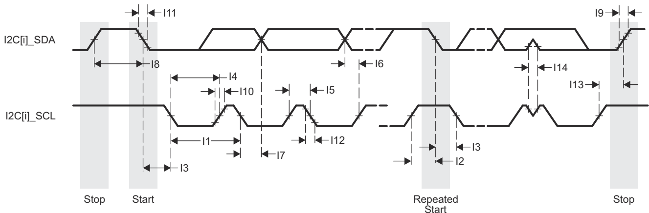
Figure 7-80. I2C Receive Timing
