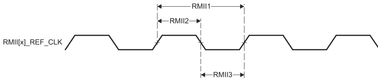
Figure 7-41. CPSW2G RMII[x]_REFCLK Timing Requirements – RMII Mode
