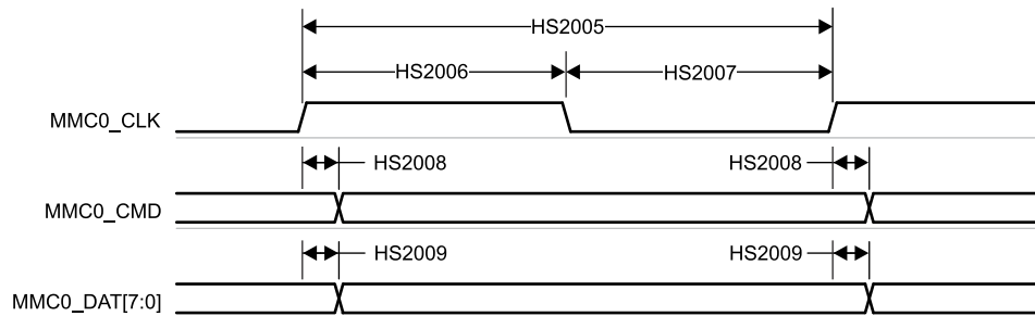
Figure 7-100. MMC0 – HS200 Mode – Transmit Mode
