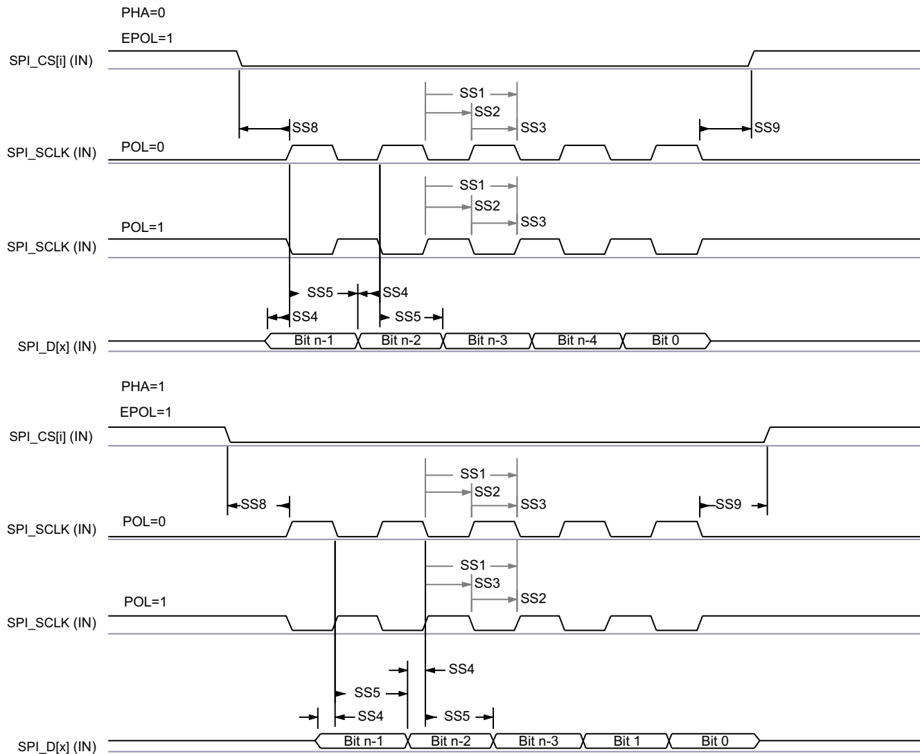
Figure 7-90. SPI Slave Mode Receive Timing
