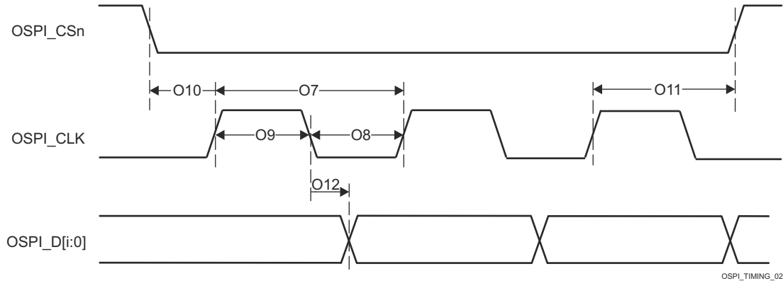
Figure 7-114. OSPI Switching Characteristics – SDR
