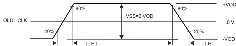
Figure 7-121. LVDS Output Transition Times
