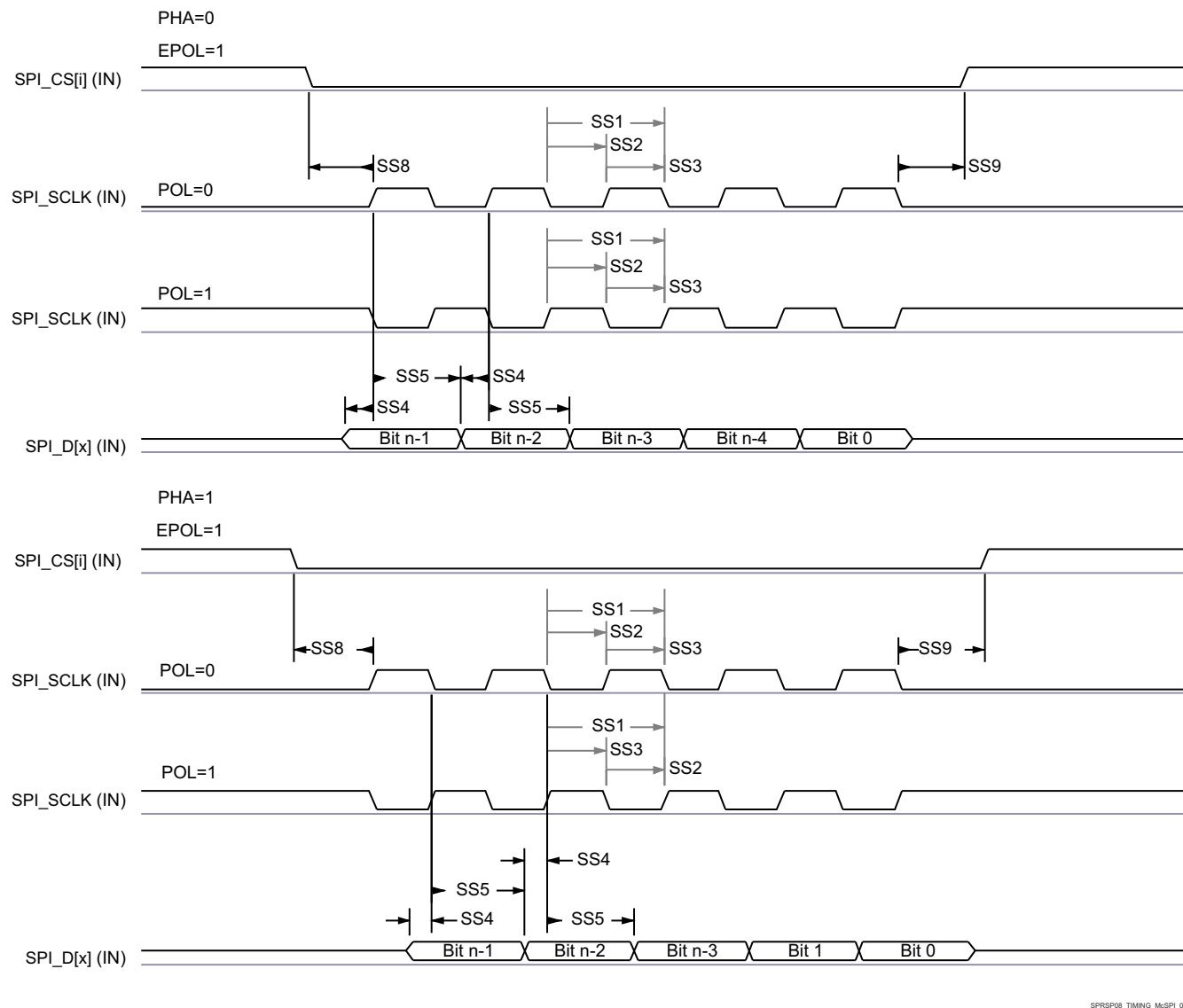
Figure 7-93. SPI Slave Mode Transmit Timing
