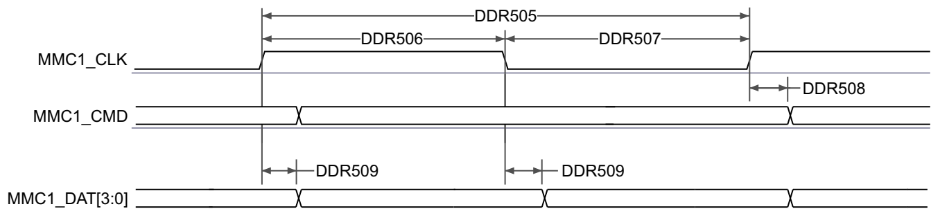
Figure 7-110. MMC1/2 – UHS-I DDR50 – Transmit Mode
