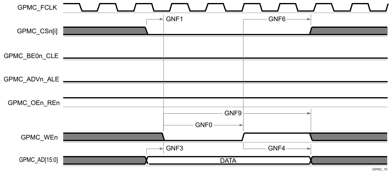
Figure 7-76. GPMC and NAND Flash — Data Write Cycle
