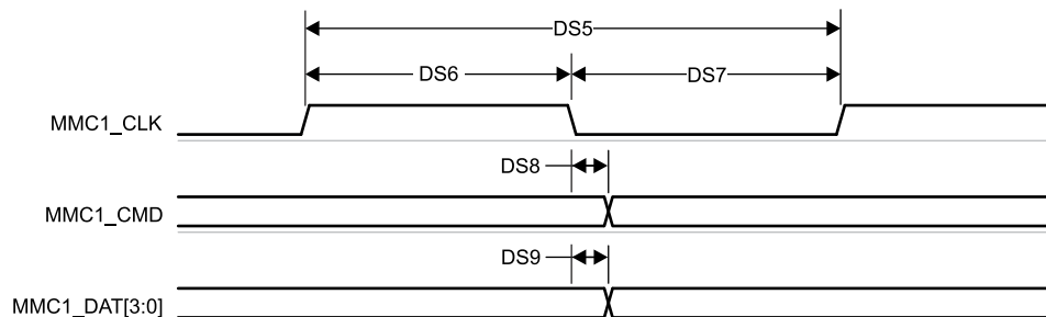
Figure 7-102. MMC1/2 – Default Speed – Transmit Mode
