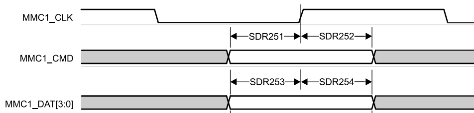
Figure 7-107. MMC1/2 – UHS-I SDR25 – Receive Mode
