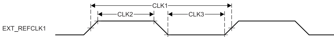
Figure 7-20. Clock Timing Requirements
