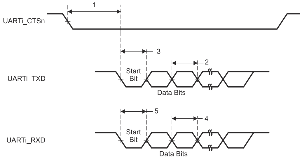
Figure 7-123. UART Timing
