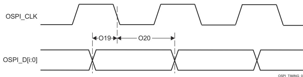
Figure 7-117. OSPI Timing Requirements – SDR, No Loopback Clock and Internal Pad Loopback Clock
