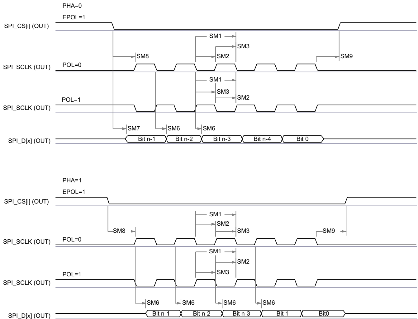
Figure 7-89. SPI Master Mode Transmit Timing
