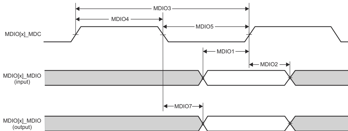
Figure 7-46. CPSW9G MDIO Diagrams Receive and Transmit
