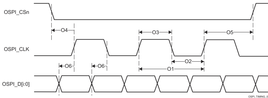
Figure 7-113. OSPI Switching Characteristics – DDR
