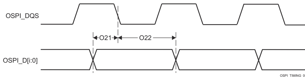
Figure 7-118. OSPI Timing Requirements – SDR, External Loopback Clock
