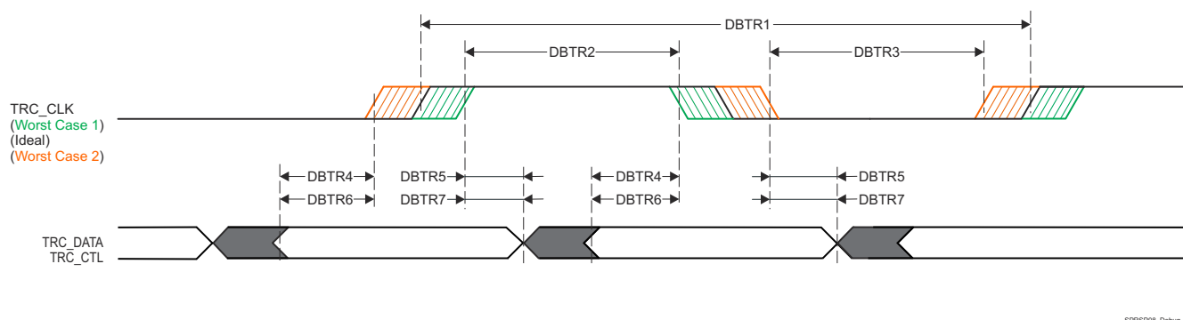
Figure 7-124. Trace Switching Characteristics
