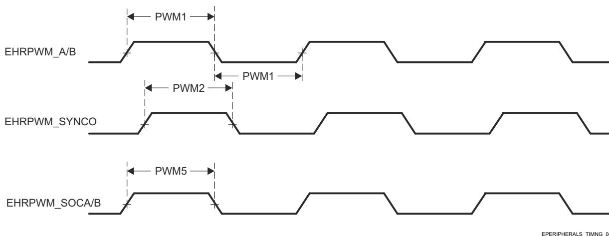
Figure 7-57. EPWM_A/B_out, ePWM_SYNC0, and ePWM_SOC/A/B Input Timings
