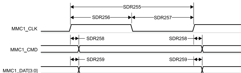
Figure 7-108. MMC1/2 – UHS-I SDR25 – Transmit Mode
