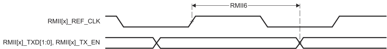
Figure 7-49. RMII[x]_TXD[1:0], and RMII[x]_TX_EN Switching Characteristics – RMII Mode
