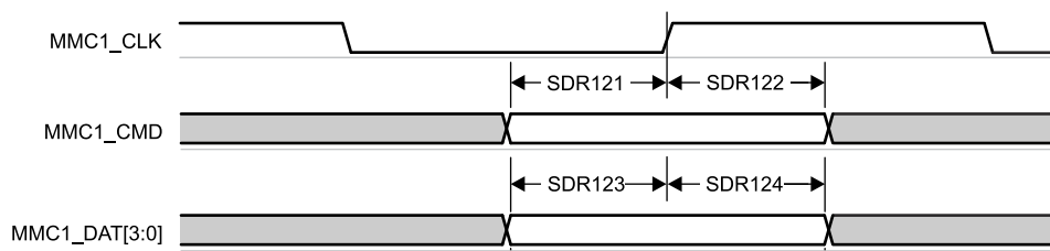
Figure 7-105. MMC1/2 – UHS-I SDR12 – Receive Mode
