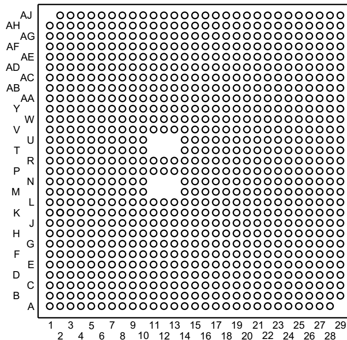
Figure 6-1. ALF FCBGA-N827 Pin Diagram (Bottom View)
