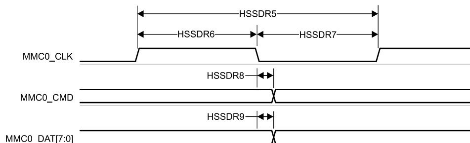
Figure 7-97. MMC0 – High Speed SDR Mode – Transmit Mode
