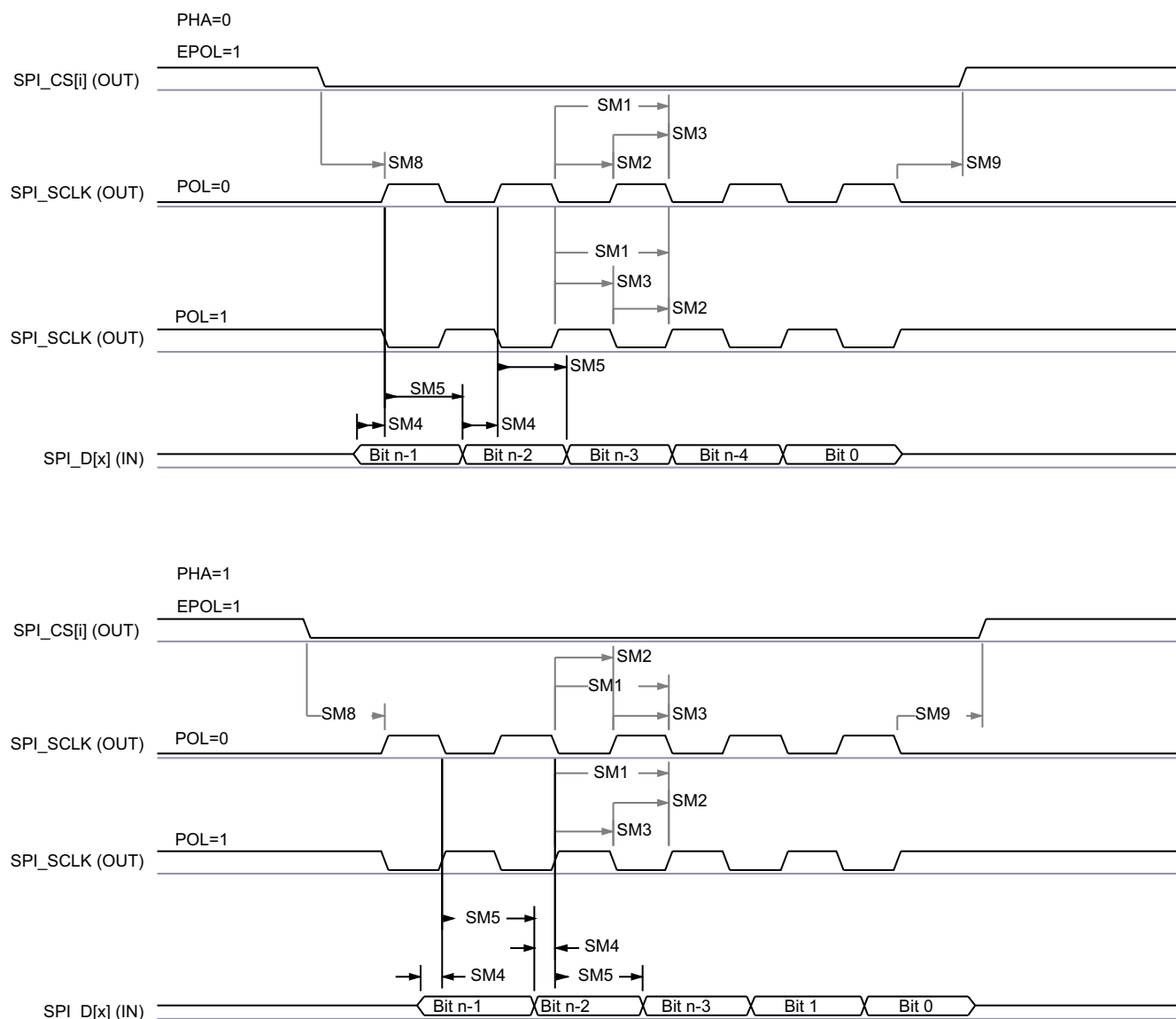
Figure 7-88. SPI Master Mode Receive Timing
