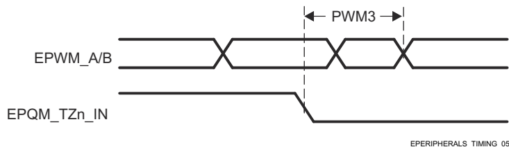
Figure 7-58. EPWM_A/B and ePWM_TZn_IN Forced High/Low Input Timings
