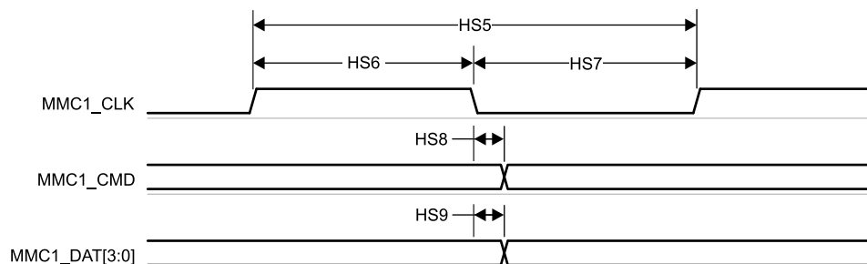
Figure 7-104. MMC1/2 – High Speed – Transmit Mode
