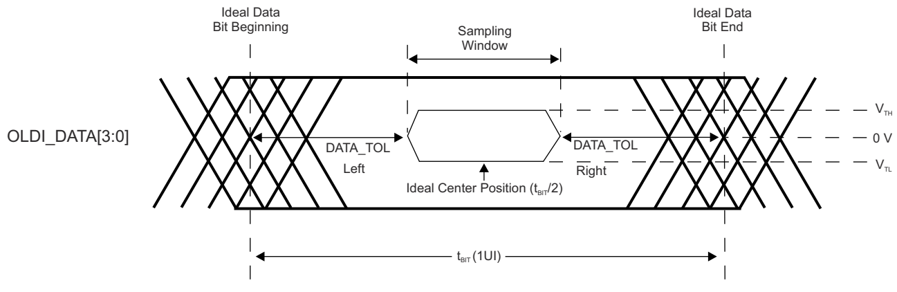
Figure 7-120. OLDI Data Output Jitter
