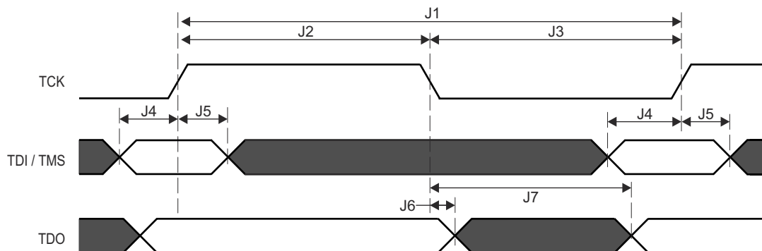
Figure 7-125. JTAG Timing Requirements and Switching Characteristics
