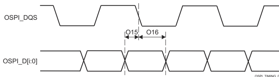
Figure 7-116. OSPI Timing Requirements – DDR, External Loopback Clock and DQS
