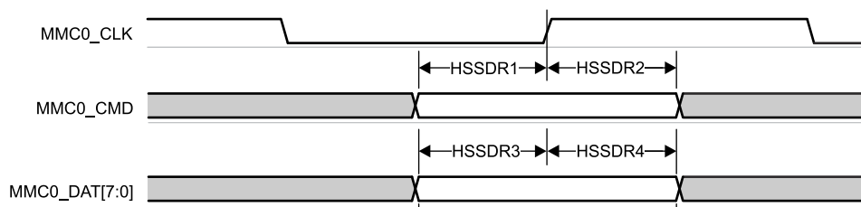
Figure 7-96. MMC0 – High Speed SDR Mode – Receive Mode
