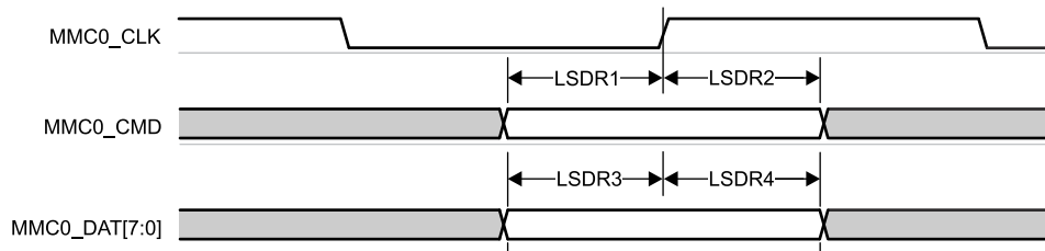
Figure 7-94. MMC0 – Legacy SDR – Receive Mode
