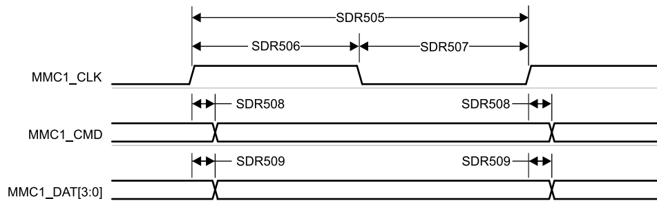
Figure 7-109. MMC1/2 – UHS-I SDR50 – Transmit Mode
