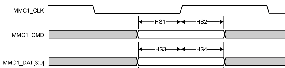
Figure 7-103. MMC1 /2- High Speed – Receive Mode
