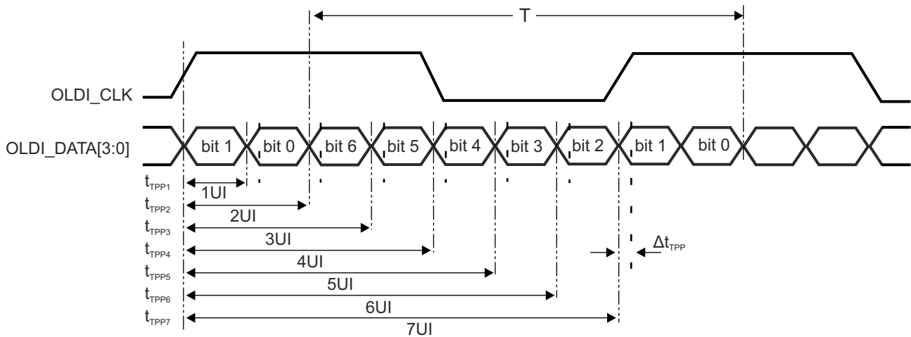
Figure 7-119. OLDI Transmitter Pulse Positions
