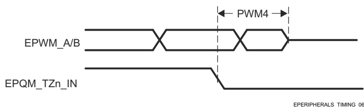
Figure 7-59. EPWM_A/B and ePWM_TZn_IN Hi-Z Input Timings
