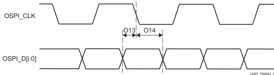
Figure 7-115. OSPI Timing Requirements – DDR, No Loopback Clock and Internal Pad Loopback Clock
