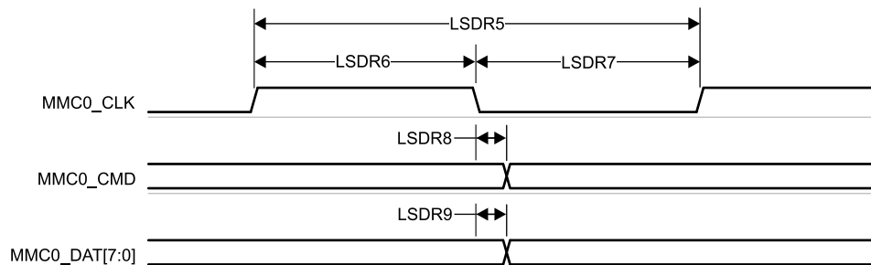
Figure 7-95. MMC0 – Legacy SDR – Transmit Mode
