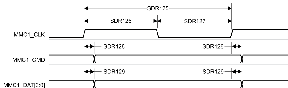
Figure 7-106. MMC1/2 – UHS-I SDR12 – Transmit Mode
