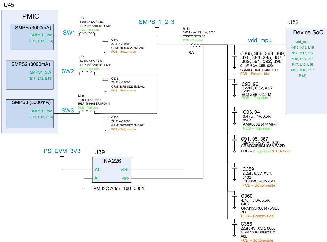
图 7-21. vdd_mpu Simplified SCH Diagram
