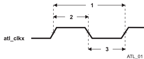
Figure 5-109. ATL_CLKOUT x Timing
