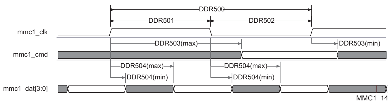
Figure 5-91. SDMMC - High-Speed SD - DDR - Data/Command Transmit
