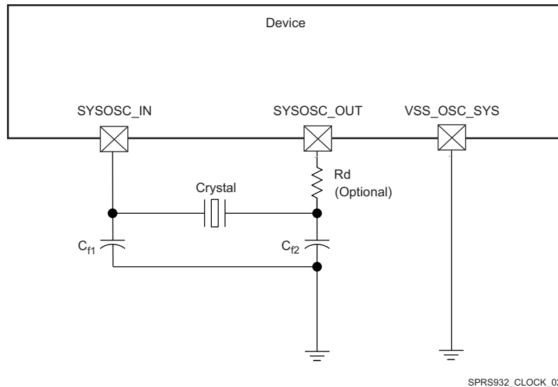
Figure 5-9. Crystal Implementation (1)
