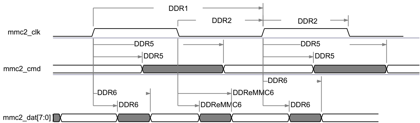
图 7-74. MMC/SD/SDIO in - High Speed DDR JC64 - Transmitter Mode
