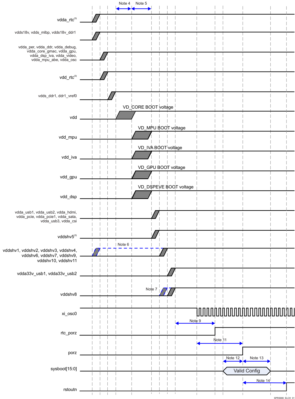
图 5-2. Power-Up Sequencing
