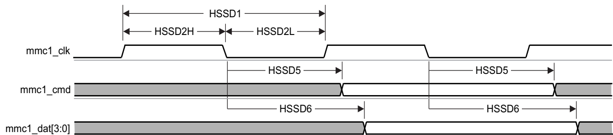
图 7-57. MMC/SD/SDIO in - High Speed - Transmitter Mode
