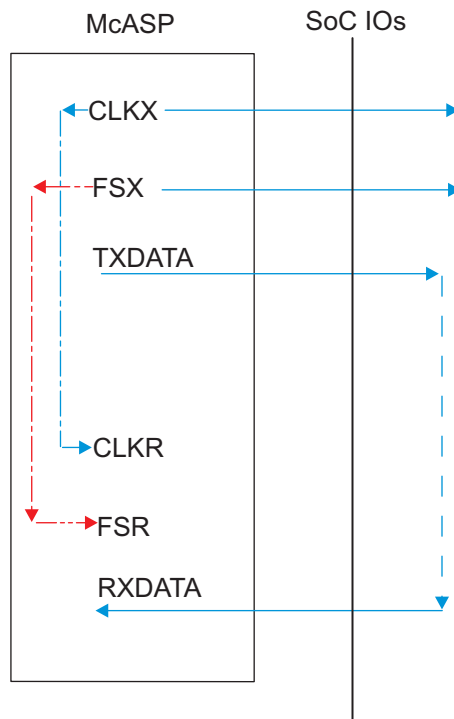
图 7-40. McASP1-8 CO-FO- - SYNC Mode
