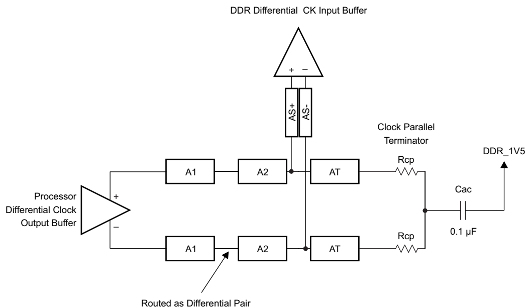
图 8-18. CK Topology for One DDR3 Device
