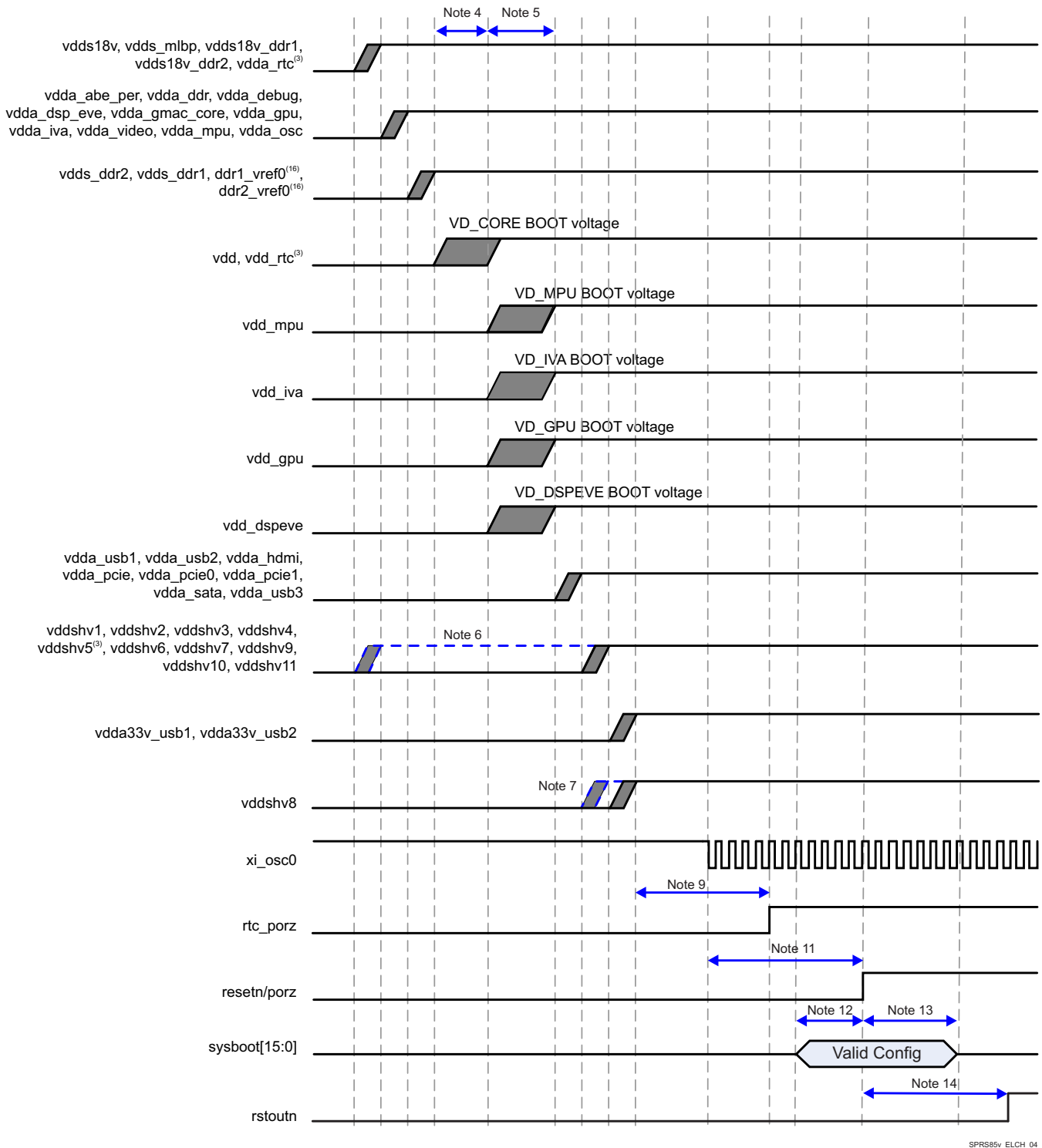
图 5-2. Power-Up Sequencing
