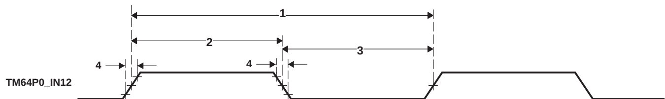
Figure 6-49. Timer Timing
