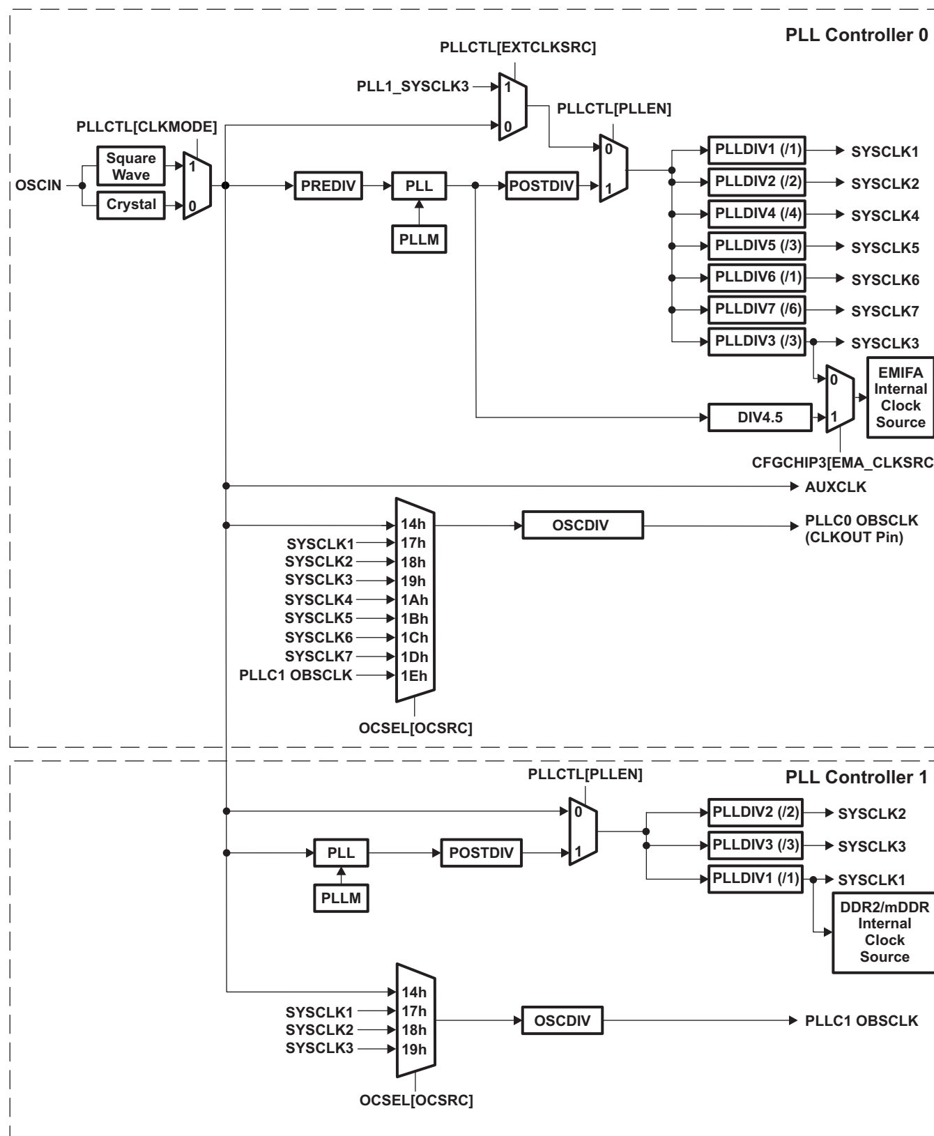
Figure 6-9. PLL Topology
