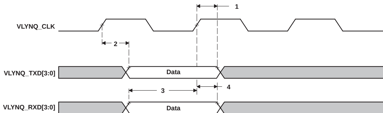
Figure 6-73. VLYNQ Transmit/Receive Timing
