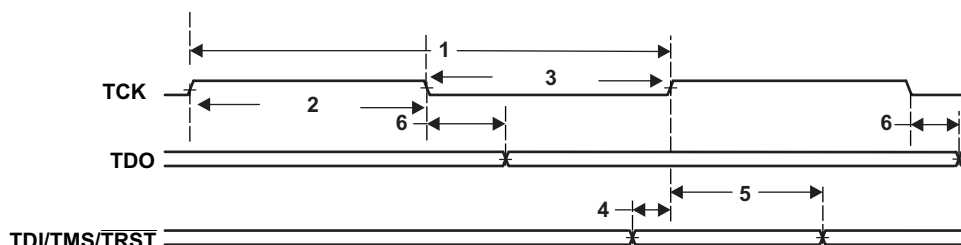
Figure 6-49. JTAG Test-Port Timing
