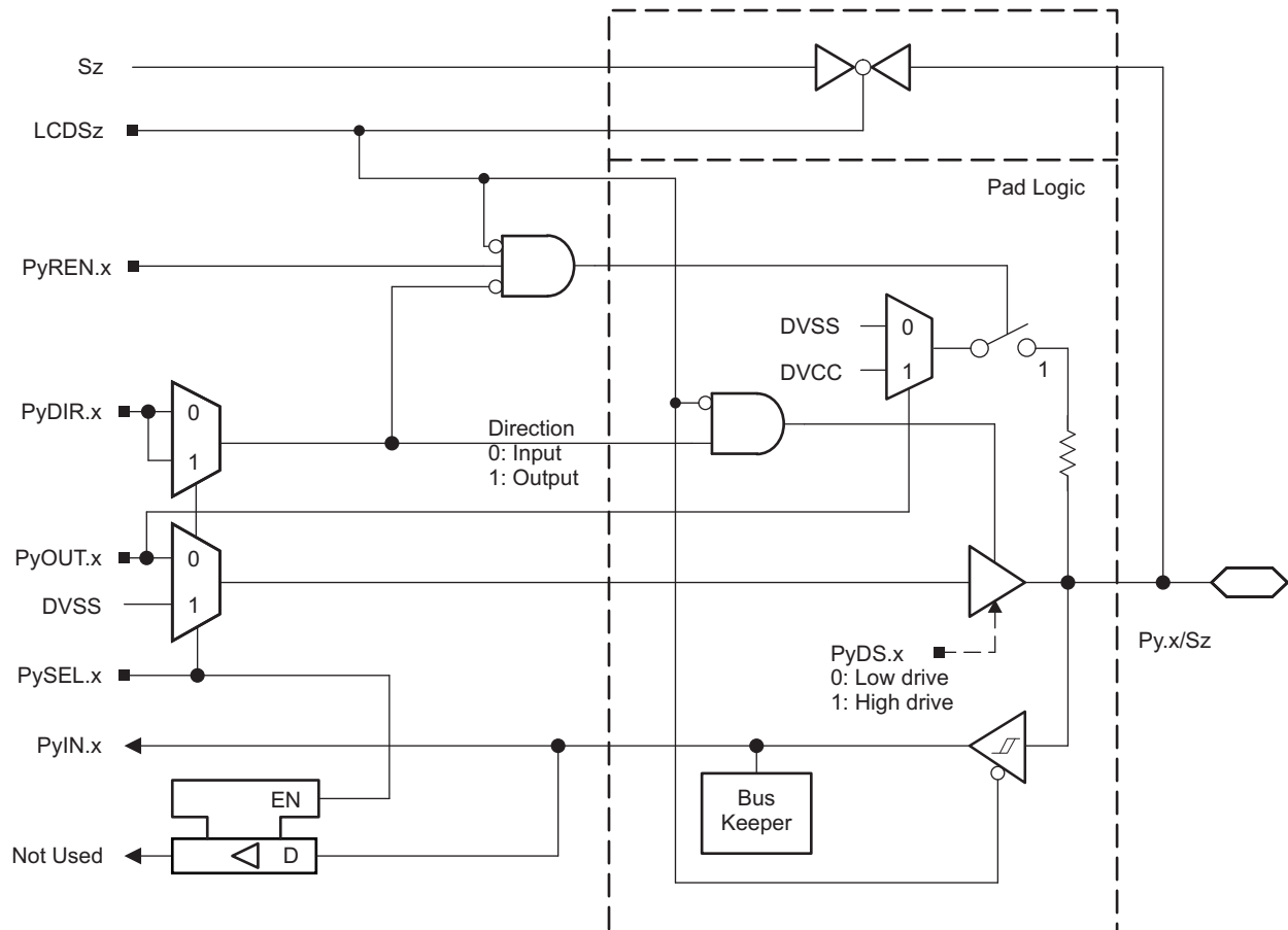
图 6-11. Port P4 (P4.0 to P4.7), Port P5 (P5.0 to P5.7), Port P6 (P6.0 to P6.7), Port P7 (P7.0 to P7.7), Port P8 (P8.0 to P8.3) Diagram (PZ Package Only)
