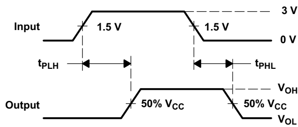
VOLTAGE WAVEFORMS
