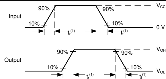
图 4. Voltage Waveforms Transition Times
