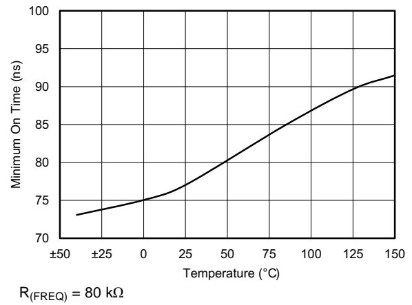
图 14. Minimum On Time vs Temperature
