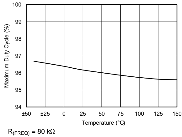
图 13. Maximum Duty Cycle vs Temperature
