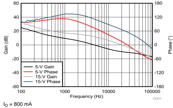
图 25. Closed Loop Gain and Phase of the Boost Converter
