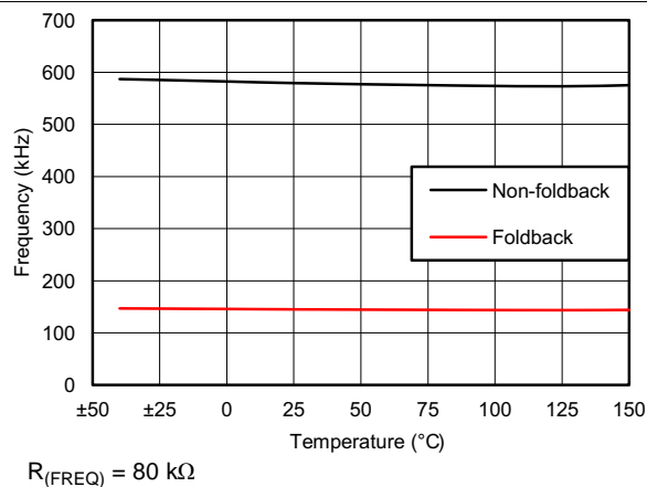
图 7. Minimum Switching Frequency for Quick Recovery from Frequency Foldback
