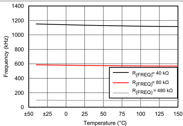
图 8. Frequency vs Temperature
