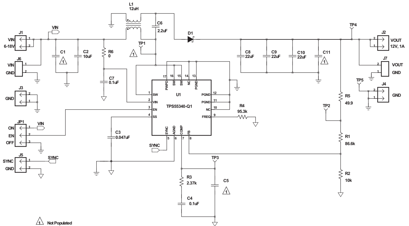
图 26. SEPIC-Converter Application Schematic
