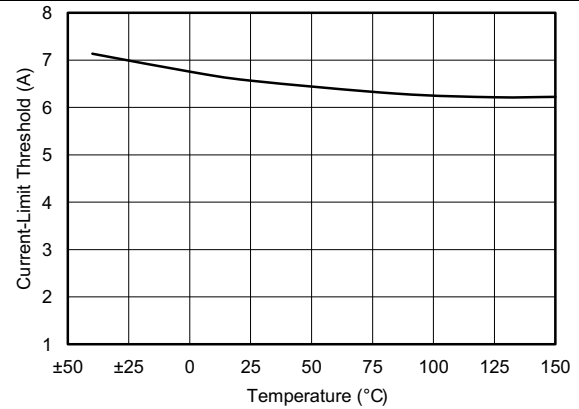
图 2. Switch Current-Limit vs Temperature
