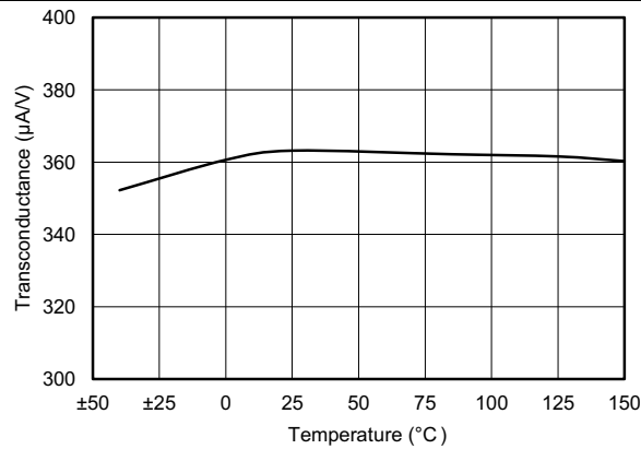
图 1. Error Amplifier Transconductance vs Temperature
