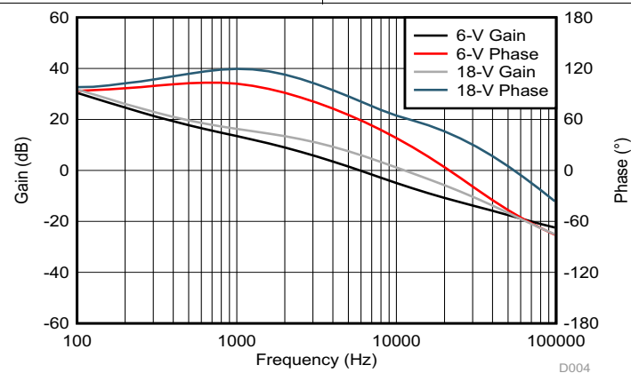
图 32. Closed Loop Gain and Phase of the SEPIC Converter
