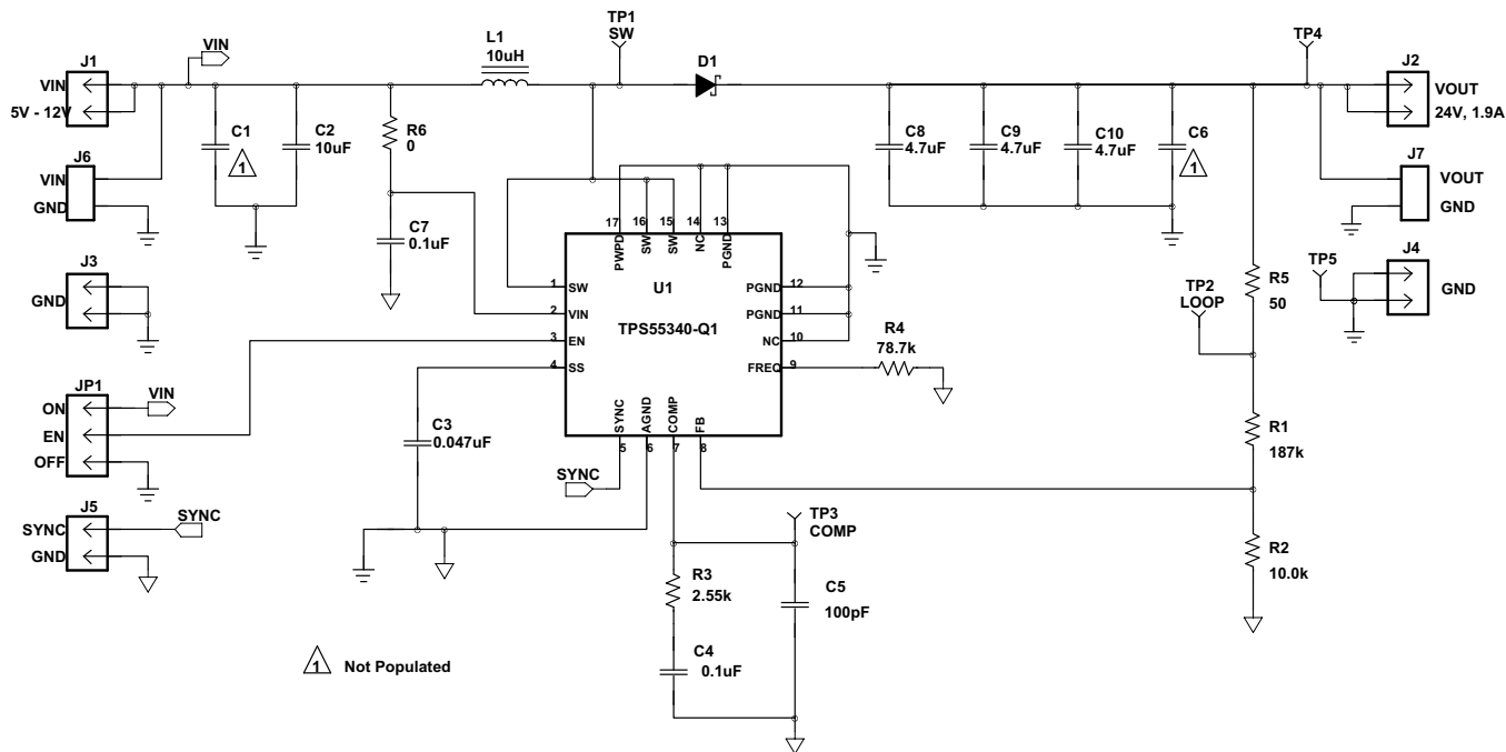
图 17. Boost Converter Application Schematic
