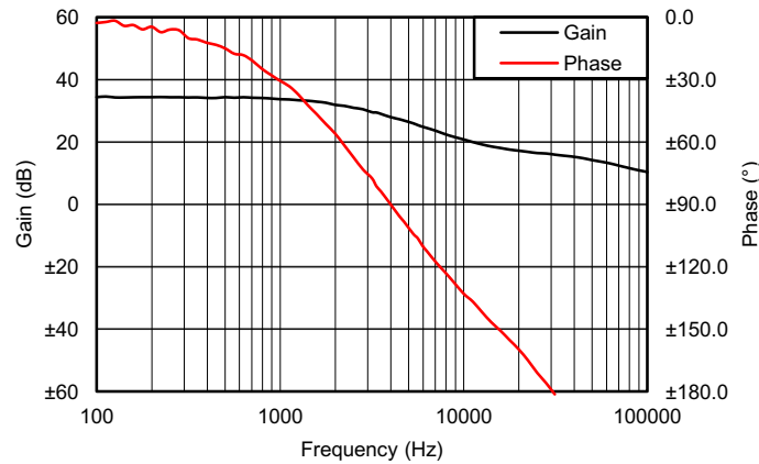
图 18. Power Stage Gain and Phase of the Boost Converter
