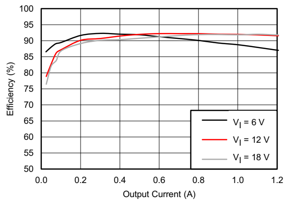
图 28. Efficiency Versus Output Current
