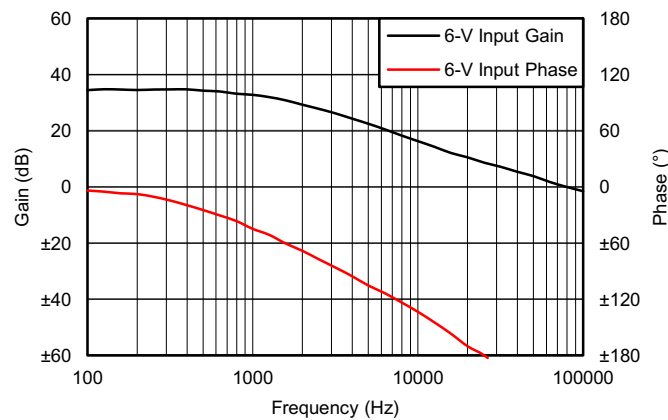
图 27. SEPIC Power Stage Gain and Phase
