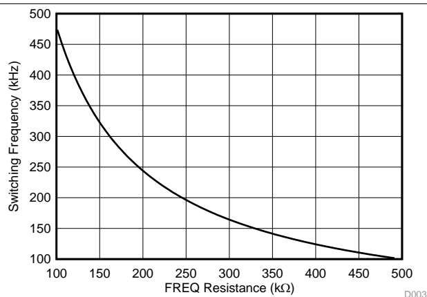
图 5. Frequency vs FREQ Resistance Low Frequency Range
