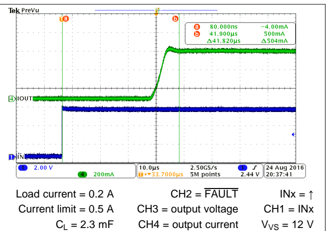
Figure 39. Driving a Capacitive Load, Expanded Waveform
