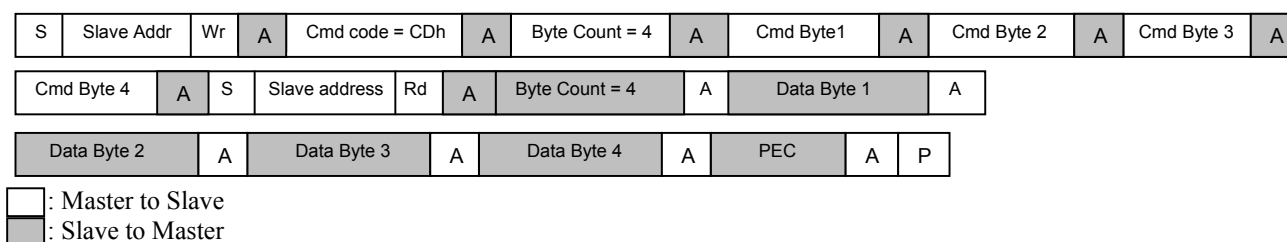
Figure 7-6 CSR Read Operation Using SMBus Block Read – Block Write Process Call with PEC
