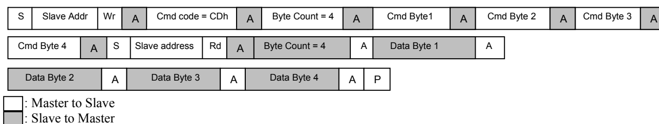
Figure 7-5 CSR Read Operation Using SMBus Block Read – Block Write Process Call
