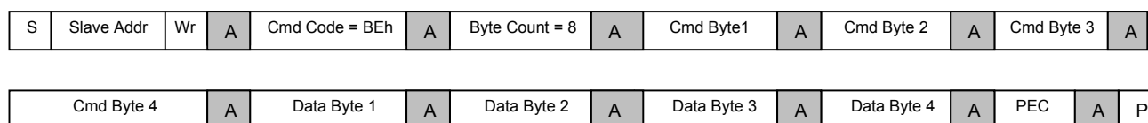
Figure 7-3 SMBus Block Write Command Format, to Write to a PI7C9X2G1224GP Register with PEC
