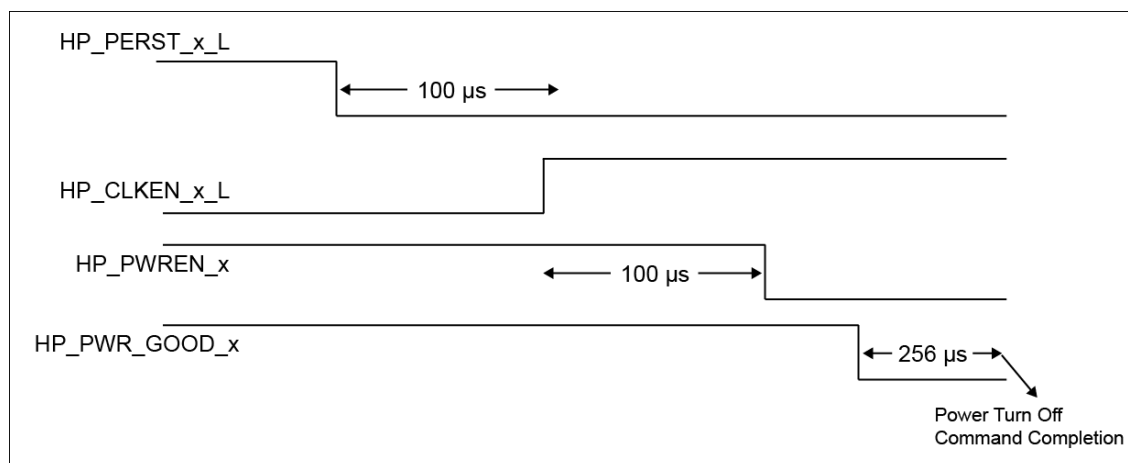
Figure 6-11 Hot Plug Automatic Power-Down Sequence
