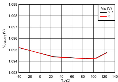
Figure 7-9. EN/UVLO Falling Threshold vs Temperature
