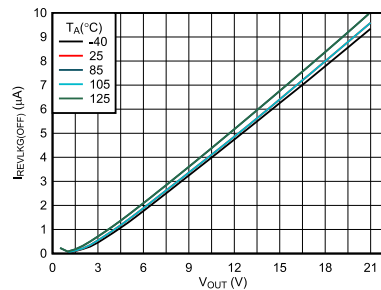
Figure 7-19. Reverse Leakage Current During OFF-State
