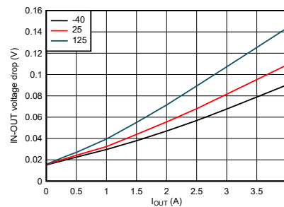
Figure 7-3. Forward Voltage Drop vs Load Current
