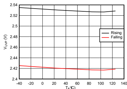
Figure 7-7. IN Undervoltage Threshold vs Temperature
