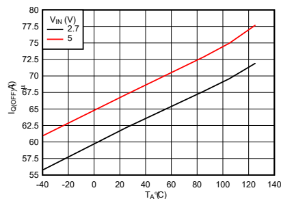
Figure 7-5. IN OFF state (UVLO) Current vs Temperature
