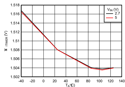
Figure 7-23. ITIMER discharge differential voltage threshold vs Temperature
