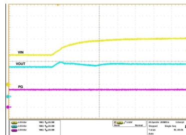
ROVSEL = \text{Open} , C_{OUT} = 220\text{ }\mu\text{F} , I_{OUT} = 150\text{ mA} , V_{IN} ramped up from 5 V to 8 V
