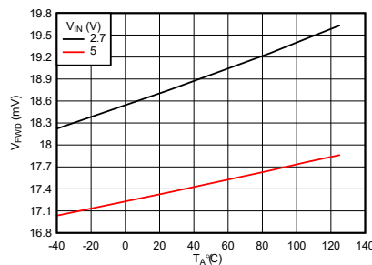
Figure 7-16. RCB - Forward Regulation Voltage vs Temperature
