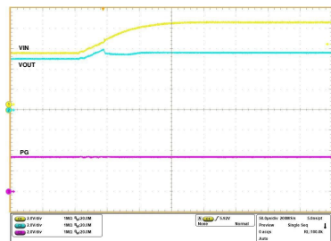
ROVSEL = GND , C_{OUT} = 220\text{ }\mu\text{F} , I_{OUT} = 120\text{ mA} , V_{IN} ramped up from 3.3 V to 6 V
