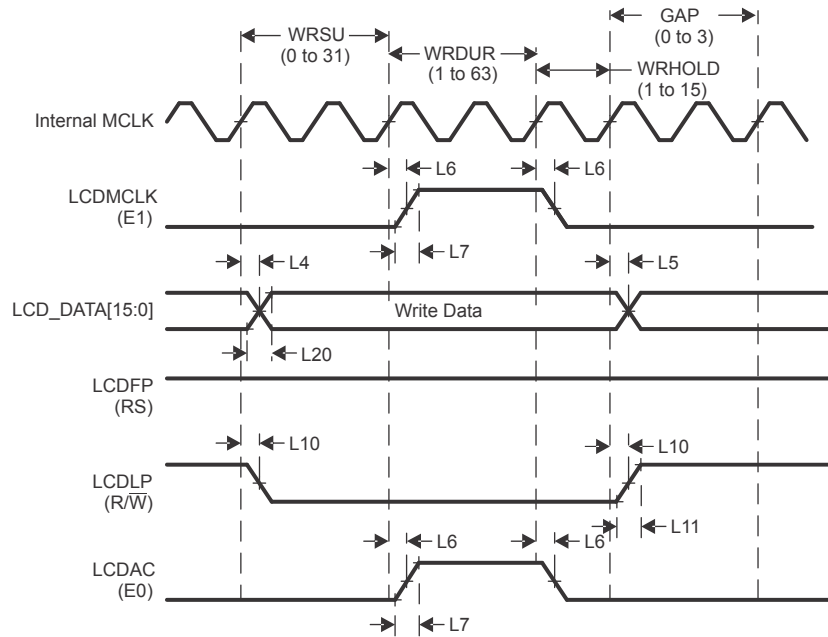
Figure 27-36. Data Write in Hitachi Mode
