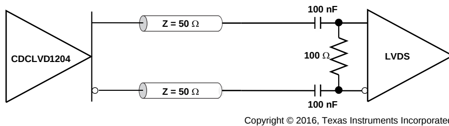
Figure 11. Output AC Termination (With the Receiver Internally Biased)
