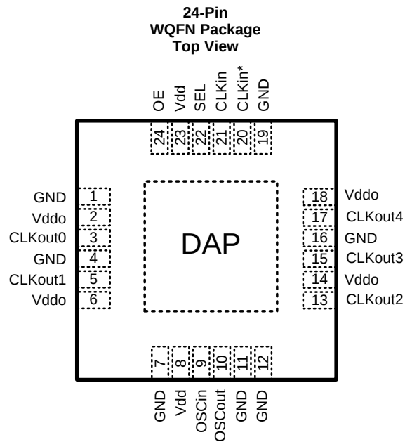
Pin Functions
