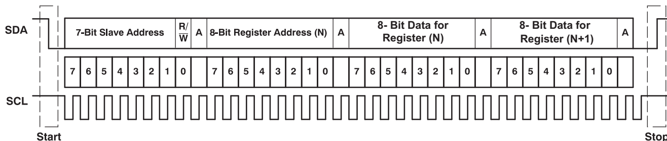
图 33. Typical I²C Sequence
