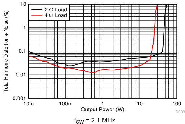
图 7-27. PBTL THD+N vs Power
