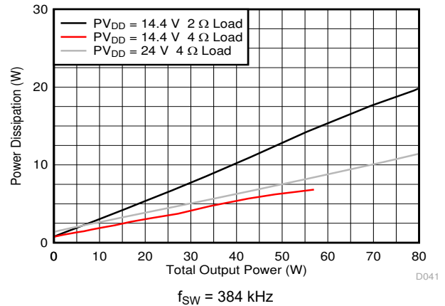
图 7-32. BTL Power Dissipation vs Total Output Power
