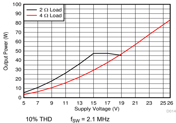
图 7-13. Output Power vs Supply Voltage
