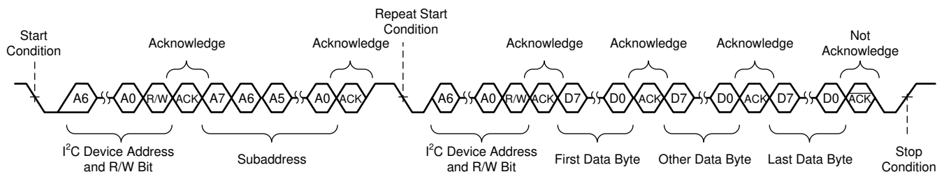
图 9-14. Sequential Read Transfer
