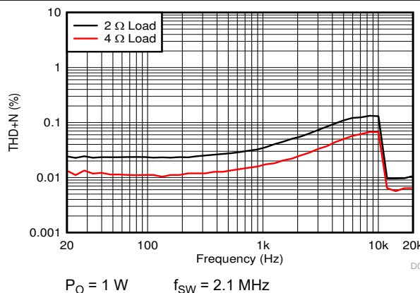
图 7-23. PBTL THD+N vs Frequency
