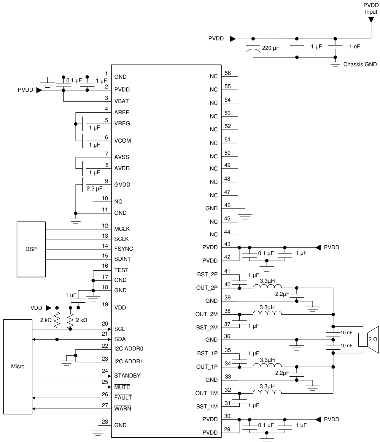
图 10-3. Typical 1-Channel PBTL Application Schematic
