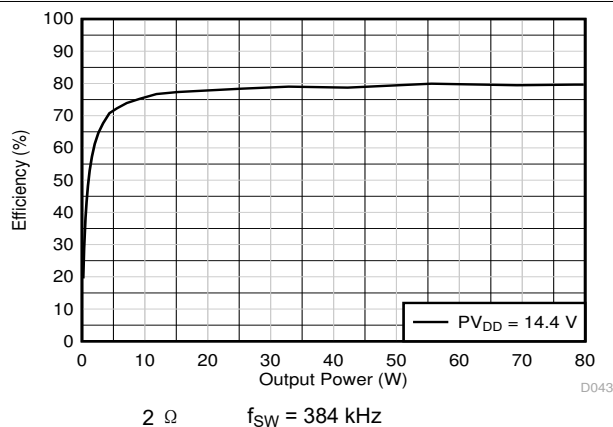
图 7-17. Power Efficiency vs Total Output Power
