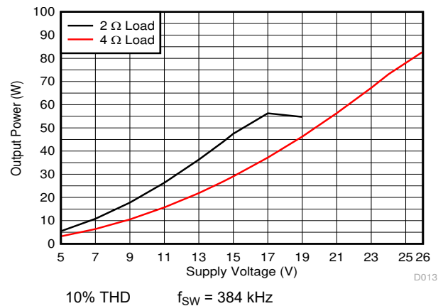
图 7-12. Output Power vs Supply Voltage
