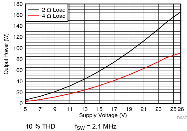
图 7-31. PBTL Output Power vs Voltage
