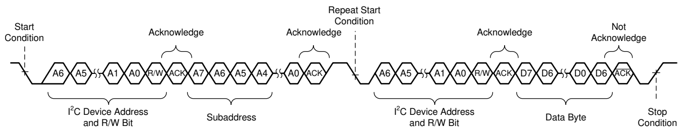
图 9-13. Random Read Transfer
