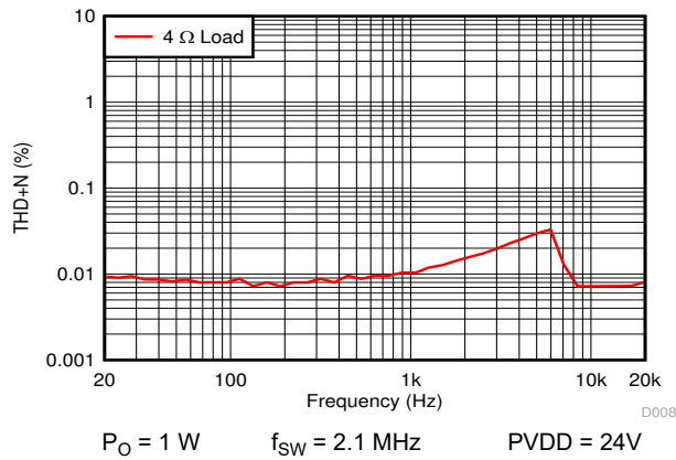
图 7-7. THD+N vs Frequency
