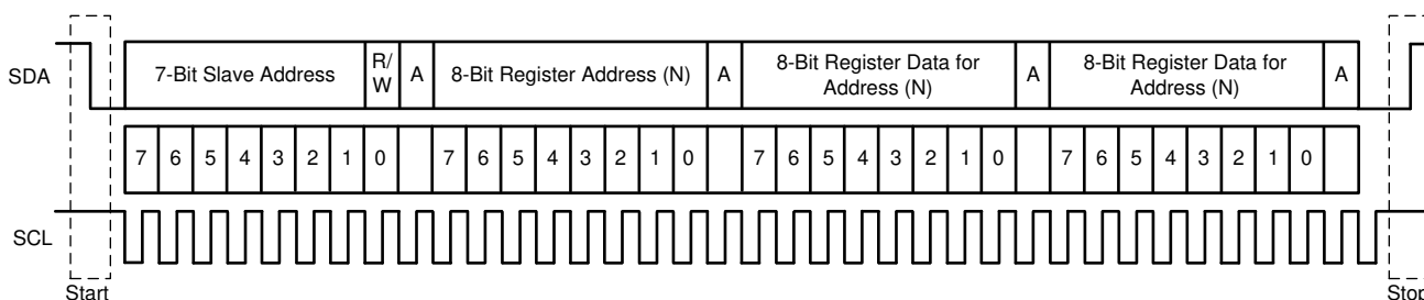
图 9-9. Typical I 2 C Sequence
