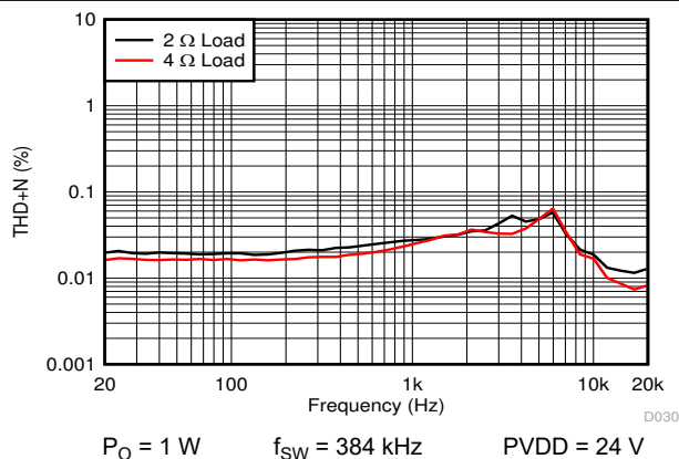
图 7-24. PBTL THD+N vs Frequency
