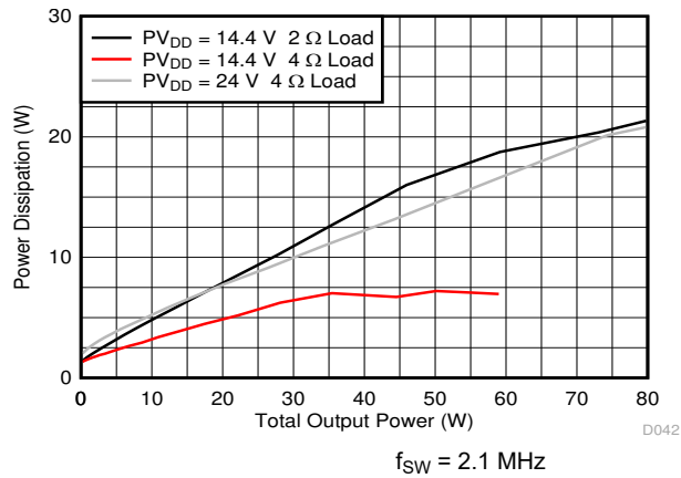
图 7-33. BTL Power Dissipation vs Total Output Power
