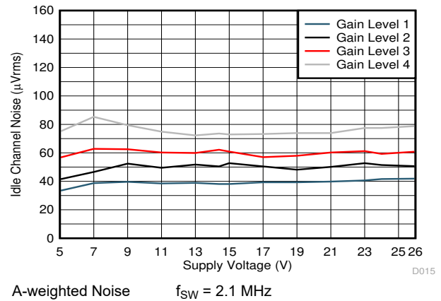
图 7-14. Noise vs Supply voltage
