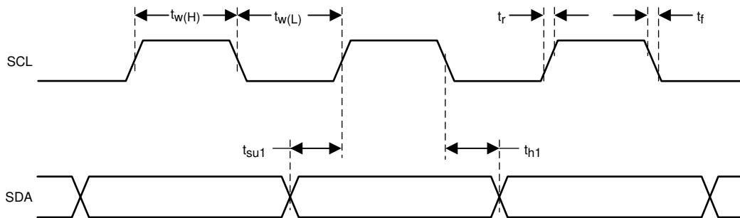
图 9-10. SCL and SDA Timing
