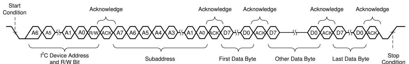
图 9-12. Sequential Write Transfer
