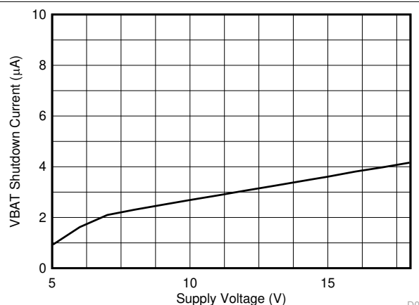
图 7-21. VBAT Standby Current vs Voltage
