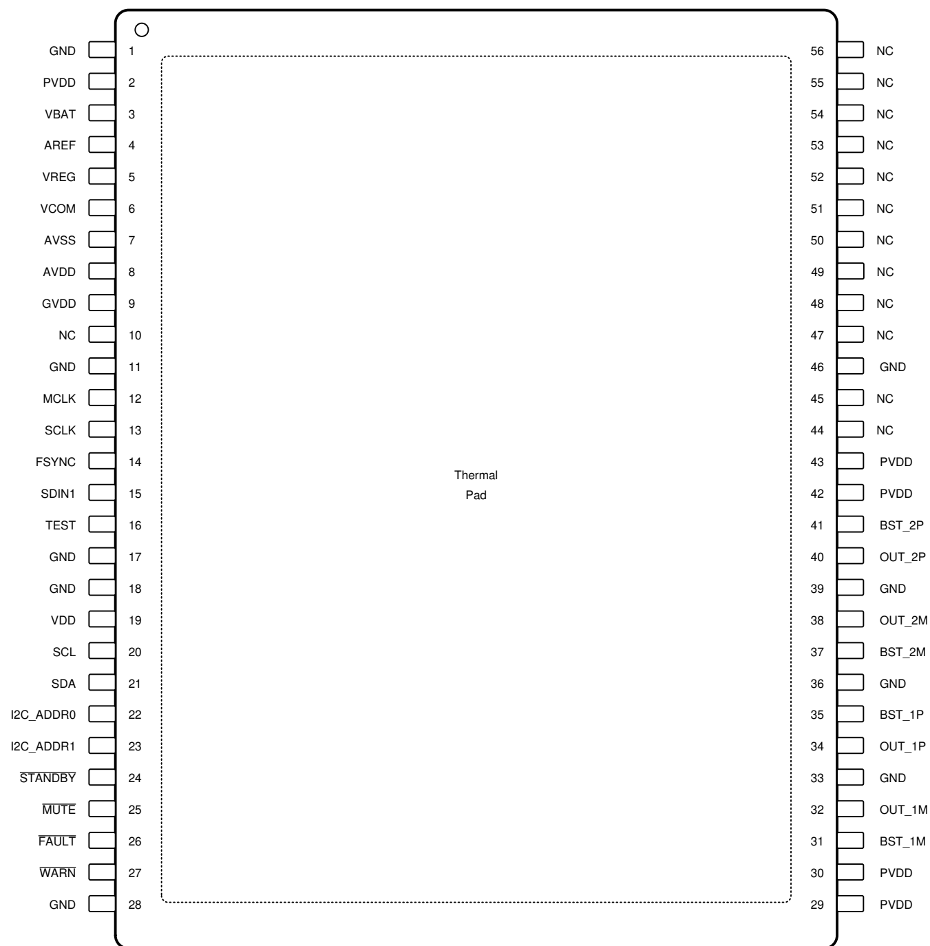
图 6-1. DKQ Package, 56-Pin HSSOP With Exposed Thermal Pad, Top View
