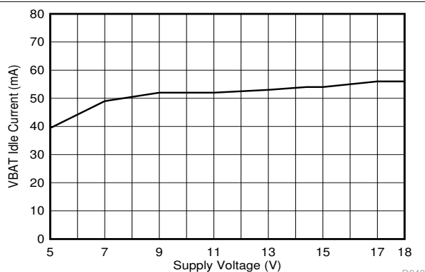
图 7-20. VBAT Idle Current vs Voltage
