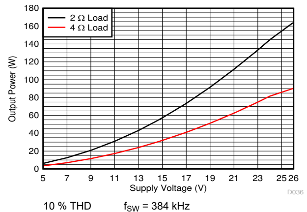
图 7-30. PBTL Output Power vs Voltage
