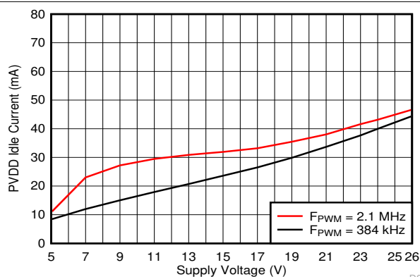
图 7-19. PVDD Idle Current vs Voltage
