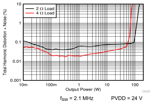
图 7-29. PBTL THD+N vs Power
