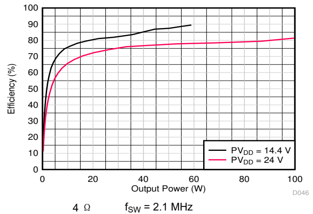
图 7-16. Power Efficiency vs Total Output Power
