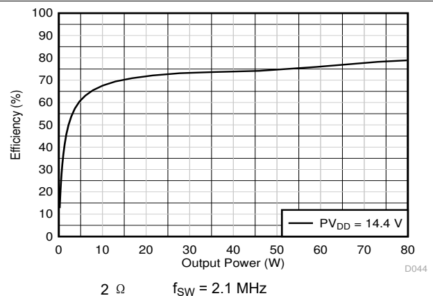
图 7-18. Power Efficiency vs Total Output Power
