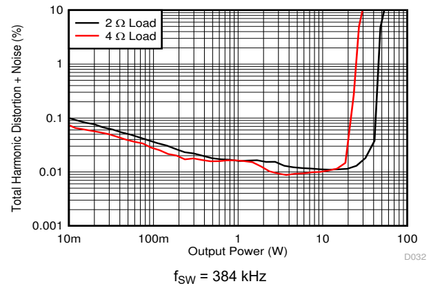
图 7-26. PBTL THD+N vs Power
