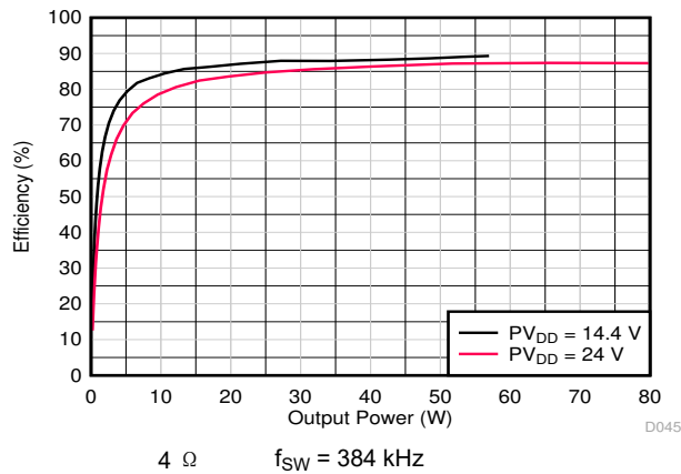
图 7-15. Power Efficiency vs Total Output Power
