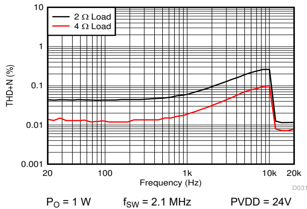
图 7-25. PBTL THD+N vs Frequency
