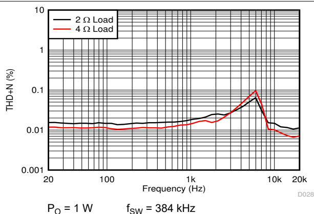
图 7-22. PBTL THD+N vs Frequency
