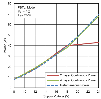
图 42. Power vs Supply Voltage (PBTL Mode)
