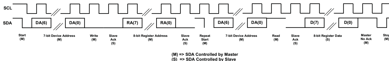
Figure 17. I²C Read
