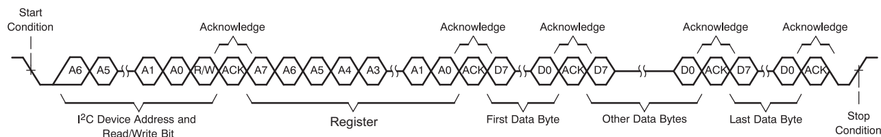
Figure 34. Multiple-Byte Write Transfer
