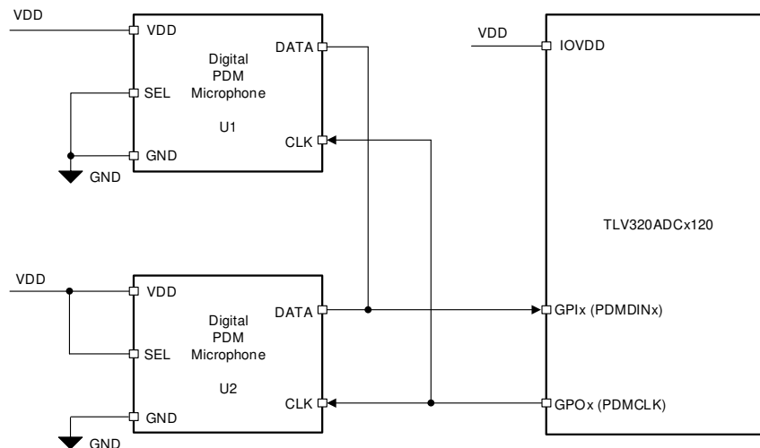
图 8-64. Digital PDM Microphones Connection Diagram to the TLV320ADC5120
