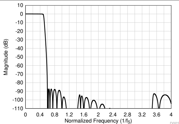
图 8-49. Ultra-Low-Latency Decimation Filter Magnitude Response
