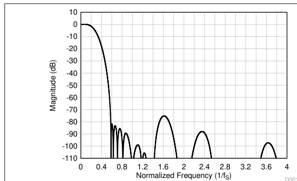
图 8-35. Linear Phase Decimation Filter Magnitude Response
