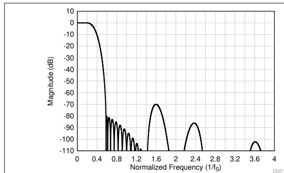
图 8-33. Linear Phase Decimation Filter Magnitude Response
