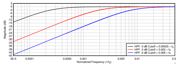
图 8-17. HPF Filter Frequency Response Plot
