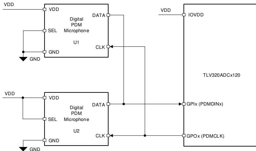
图 8-64. Digital PDM Microphones Connection Diagram to the TLV320ADC3120
