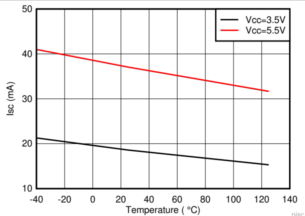
Figure 6-19. Output Short-Circuit (Source) Current vs Temperature
