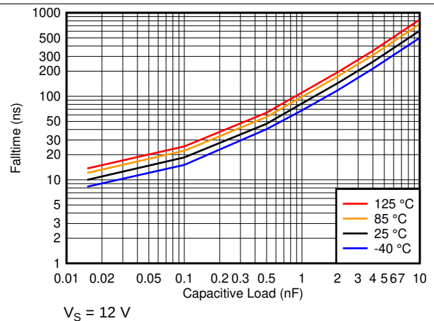
图 56. t_{\text{FALL}} vs. Capacitive Load at 12V
