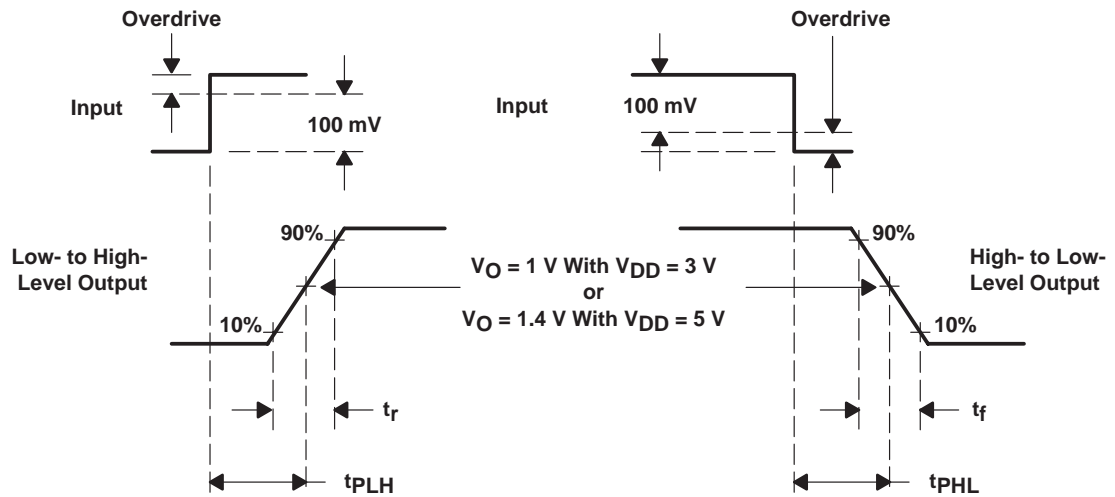
VOLTAGE WAVEFORMS
