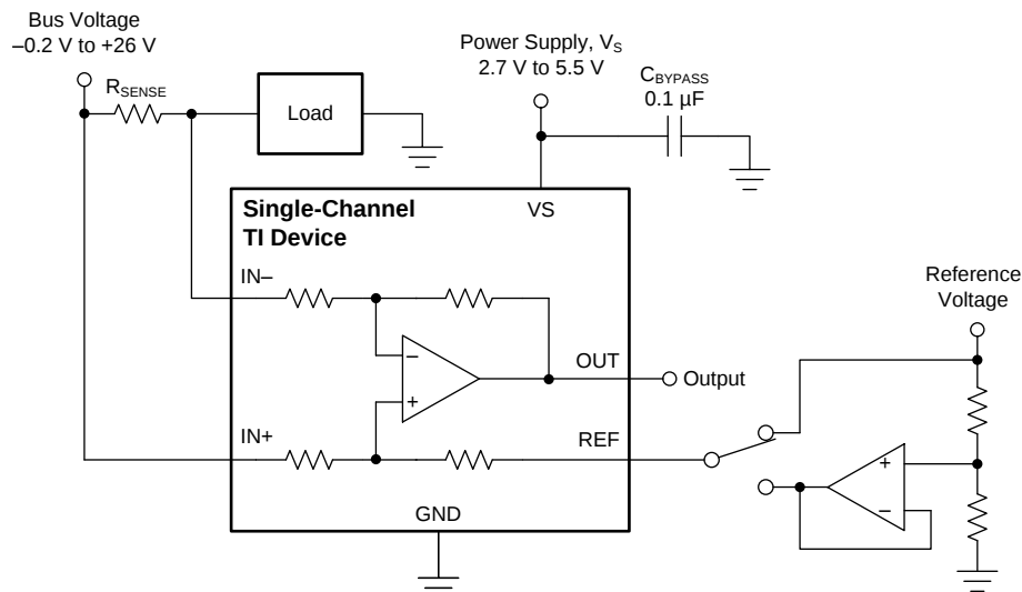
图 45. Bidirectional Application
