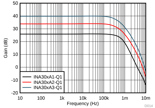
图 14. Gain vs Frequency
