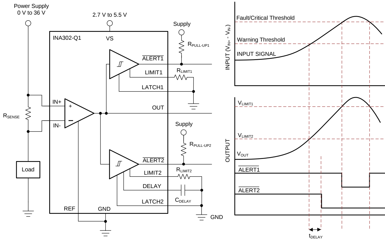
图 42. Out-of-Range Alert Responses for the INA302-Q1
