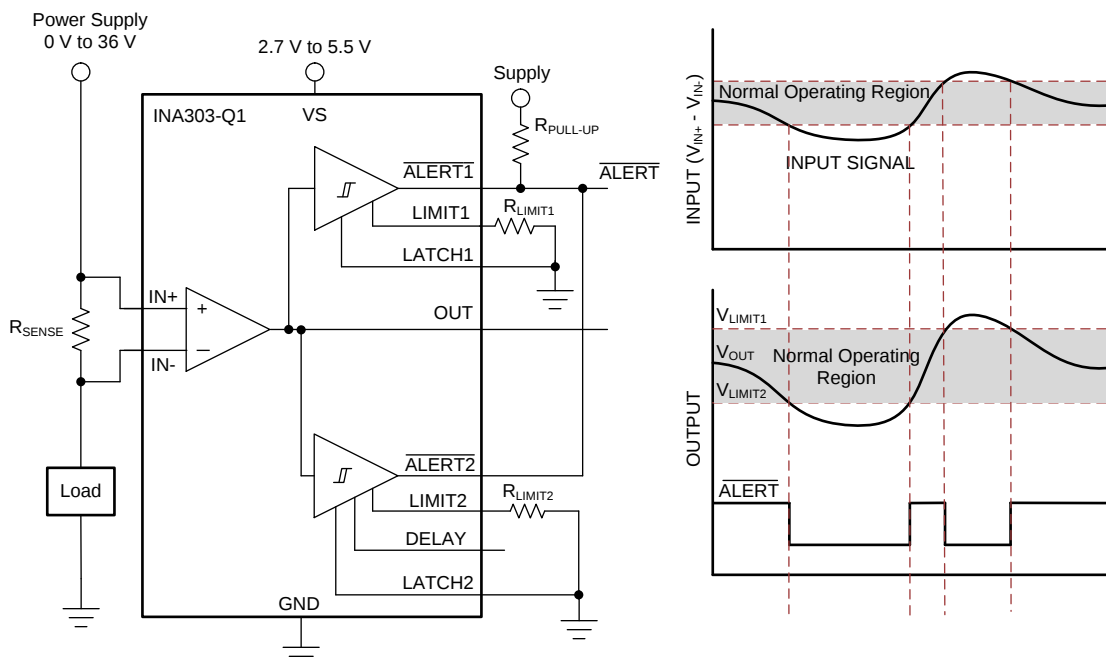
图 44. Current Window Comparator Implementation With the INA303-Q1
