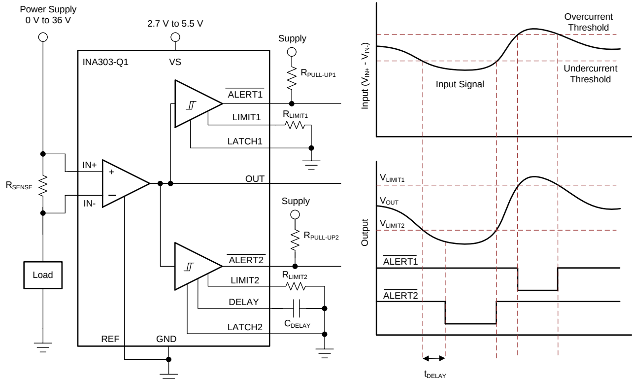
图 43. Out-of-Range Alert Responses for the INA303-Q1
