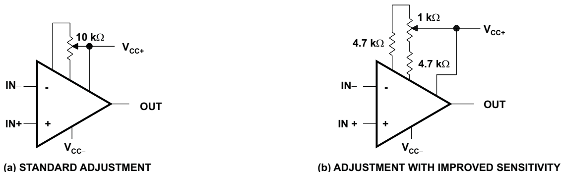
Figure 45. Input Offset Voltage Nulling Circuits
