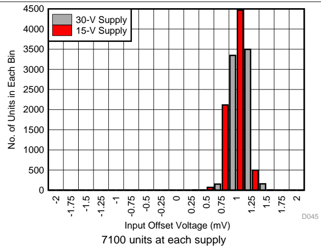
图 32. Input Offset Voltage Distribution
