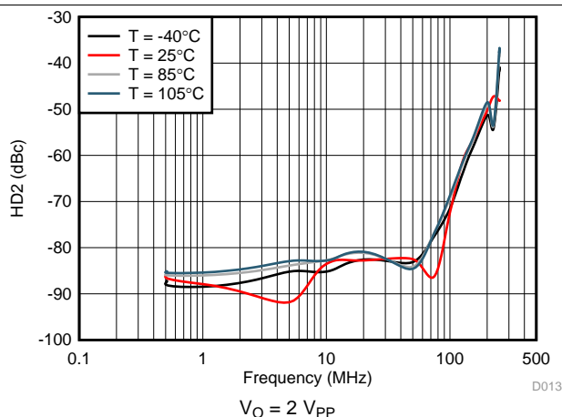
图 15. HD2 vs Frequency Across Temperature
