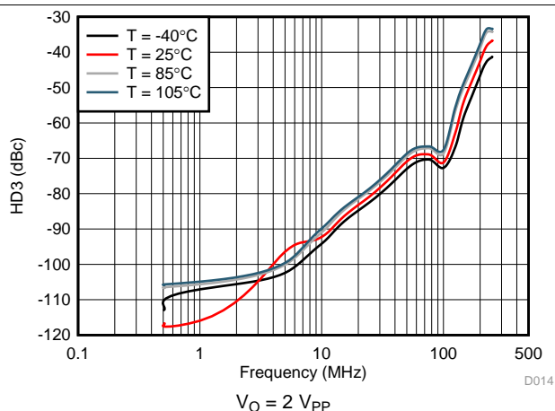
图 16. HD3 vs Frequency Across Temperature
