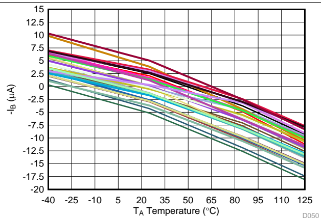
图 34. Noninverting I_B Distribution
