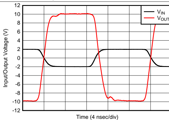
图 26. G = -5 V/V Pulse Response
