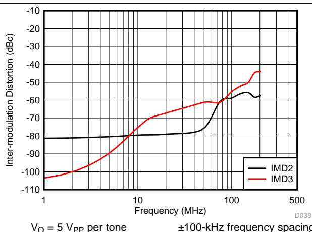
图 18. Intermodulation Distortion vs Frequency
