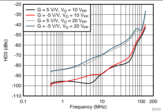
图 10. HD3 vs Frequency
