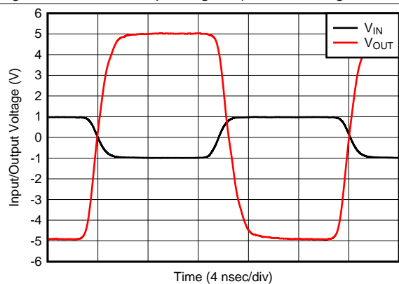
图 25. G = -5 V/V Pulse Response
