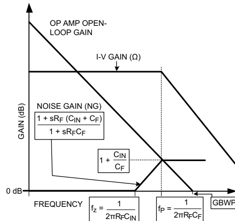
Figure 56. Transimpedance Amplifier Graphical Stability Analysis and Compensation
