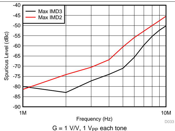
图 33. IMD2 and IMD3 vs Frequency
