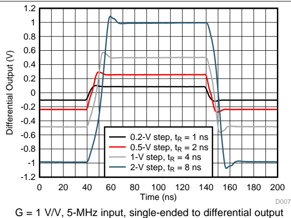
图 7. Small- and Large-Signal Step Response
