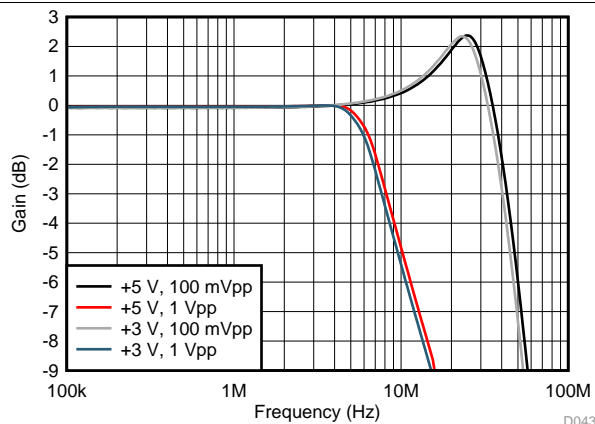
图 43. Common-Mode Voltage, Small- and Large-Signal Response (VOCM Pin Driven)
