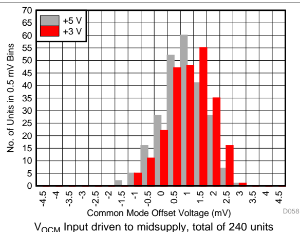
图 58. Common-Mode Output Offset from Driven V_{\text{OCM}} Histogram
