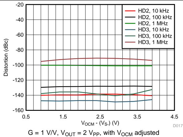
图 17. Harmonic Distortion vs V_{\text{OCM}}
