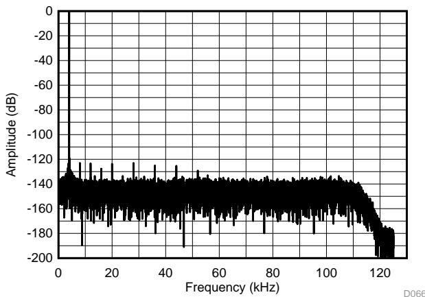
图 79. 4-kHz FFT Test for the Gain of 1 V/V Interface in 图 78
