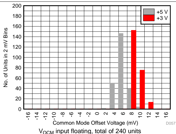
图 57. Common-Mode Output Offset from V_{\text{S+}} / 2 Default Value Histogram
