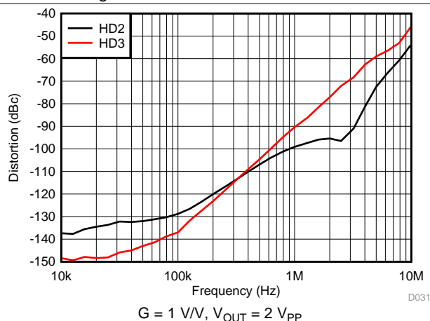
图 31. Harmonic Distortion vs Frequency
