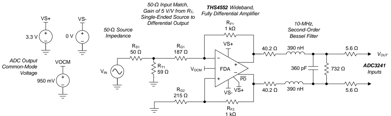
图 96. ADC3k Driver with a 2nd-Order RLC Interstage Filter
