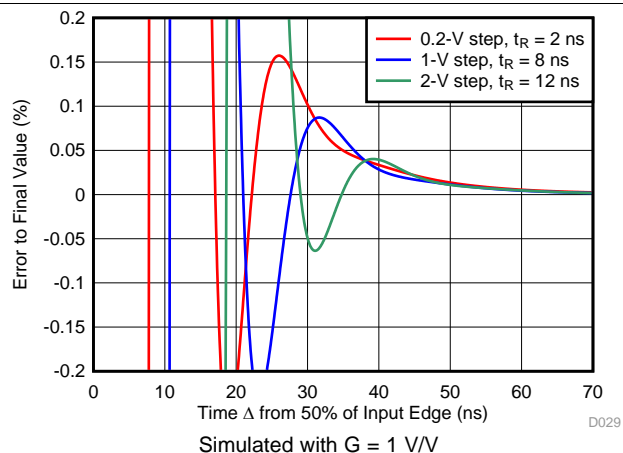
图 29. Small- and Large-Signal Step Settling Time
