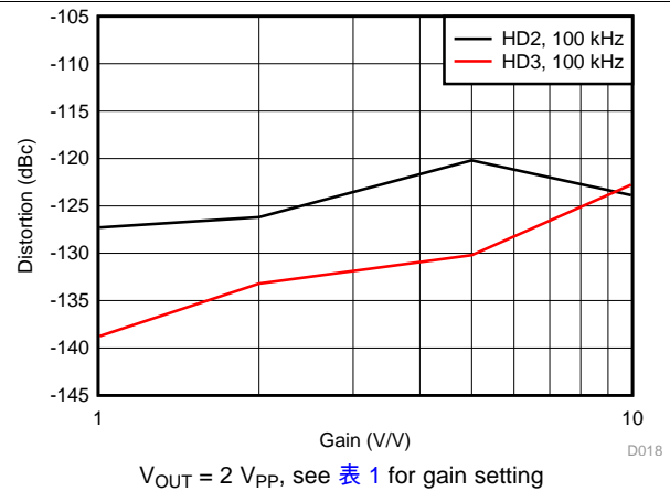
图 18. Harmonic Distortion vs Gain
