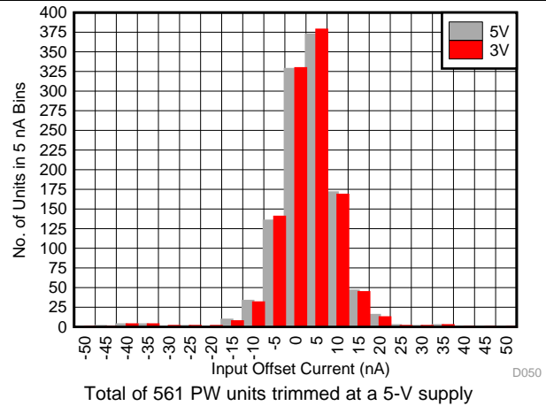
图 50. Input Offset Current ( I_{\text{OS}} )
