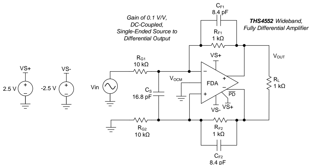
图 84. Compensated Attenuator Circuit Using the THS4552
