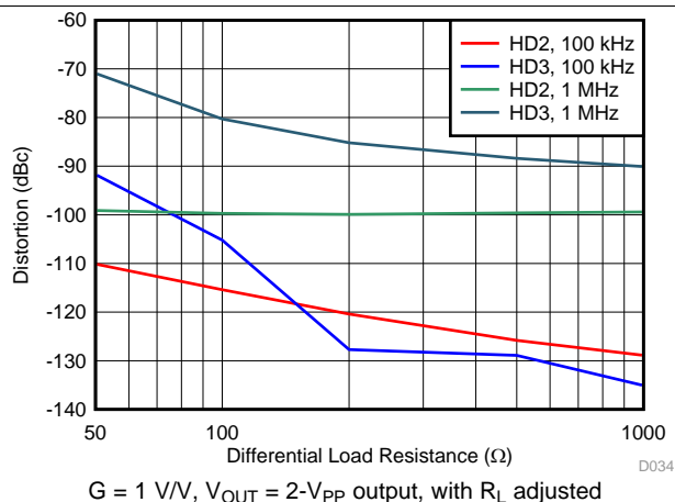
图 34. Harmonic Distortion vs R_L
