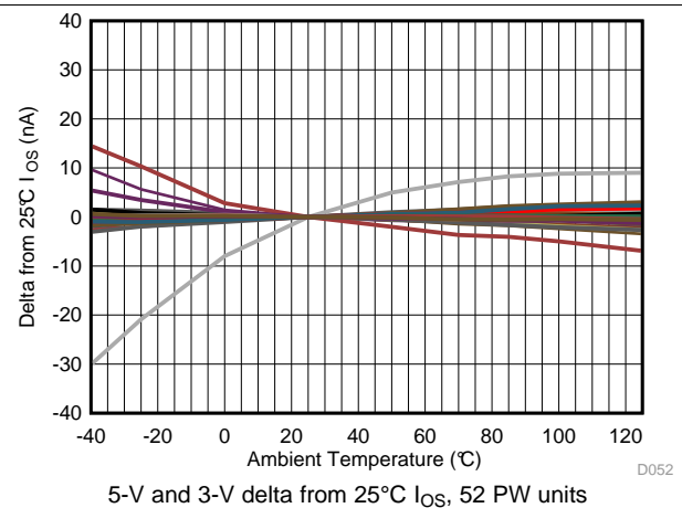
图 52. Input Offset Current vs Temperature
