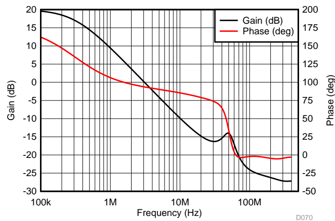
图 87. Gain and Phase Plot with a Feedback Pole
