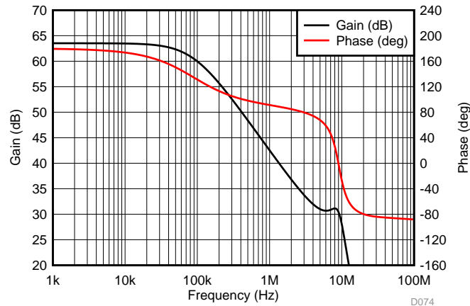
图 94. Gain and Phase Plot of DAC Output Driver
