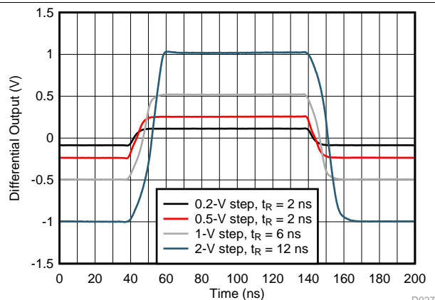
图 25. Small- and Large-Signal Step Response
