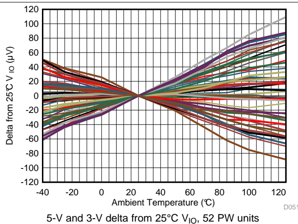
图 51. Input Offset Voltage vs Temperature
