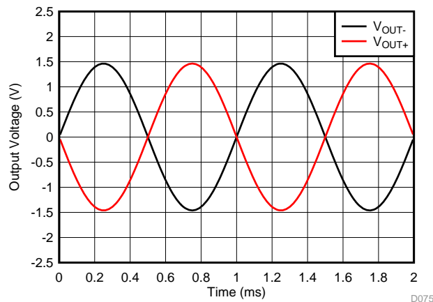
图 95. Output Waveform of the DAC Output Driver
