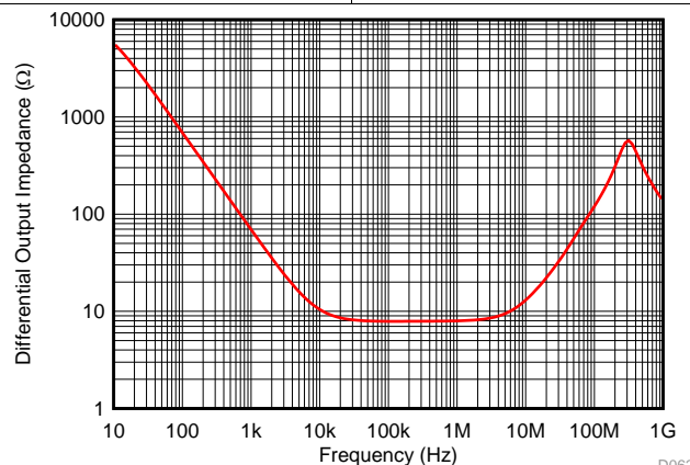
图 68. Differential Open-Loop Output Impedance
