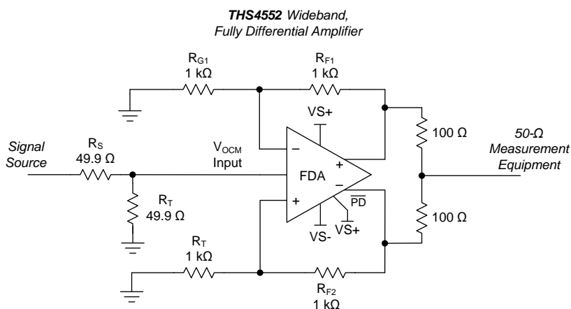
图 65. Output Common-Mode Measurements
