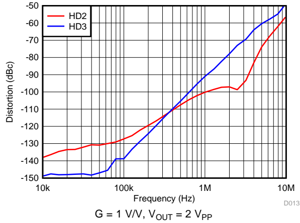
图 13. Harmonic Distortion vs Frequency
