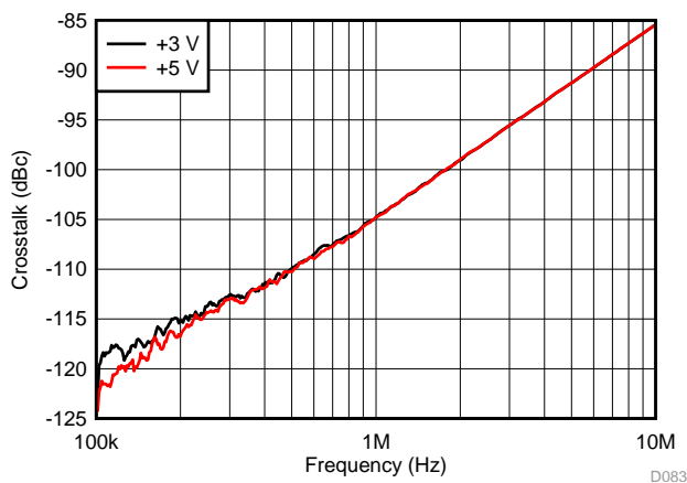
图 80. THS4552PW Crosstalk vs Frequency
