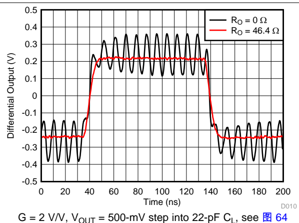
图 10. Step Response Into Capacitive Load
