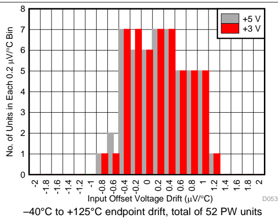
图 53. Input Offset Voltage Drift Histogram
