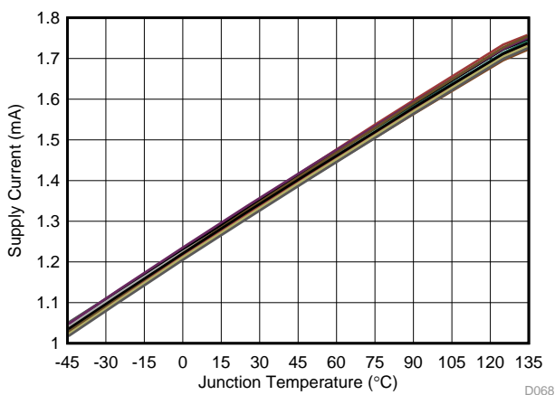
图 98. Linear Temperature Coefficient for Supply Current
