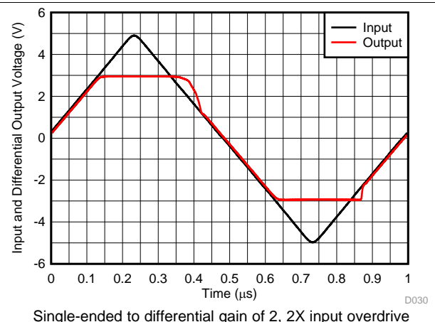
图 30. Overdrive Recovery Performance
