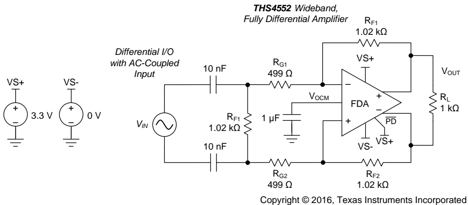
图 75. Example AC-Coupled Differential Input Design
