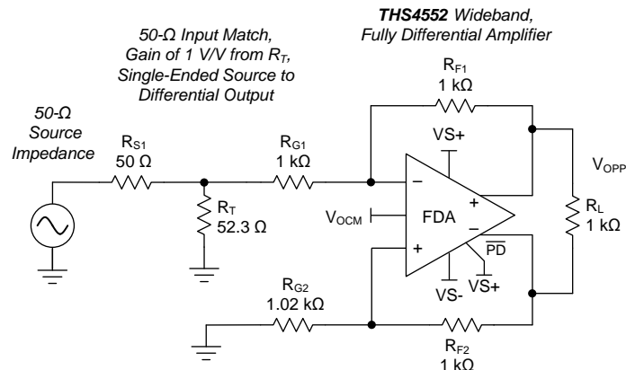
图 69. Single-Ended to Differential Gain of 1 V/V with Input Matching Using Standard Resistor Values
