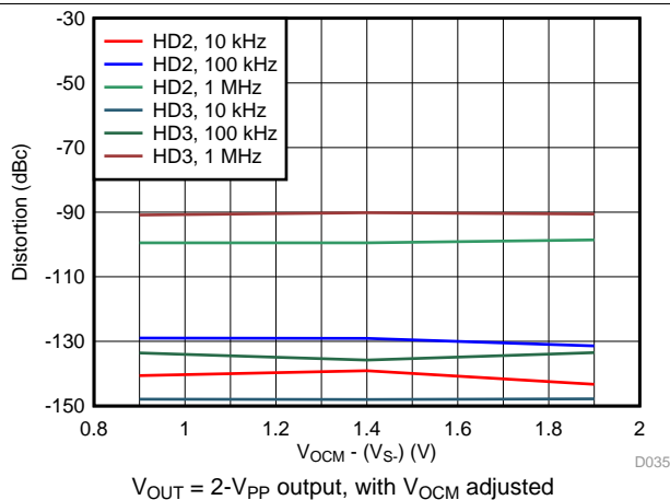
图 35. Harmonic Distortion vs V_{OCM}
