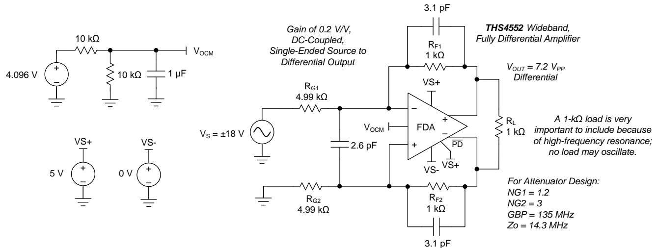
图 71. DC-Coupled, Single-Ended to Differential Attenuator Design
