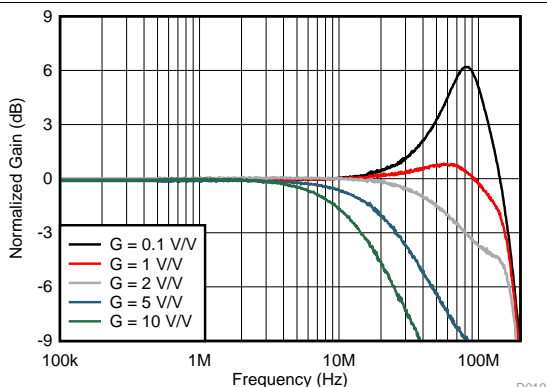
图 19. Small-Signal Frequency Response vs Gain
