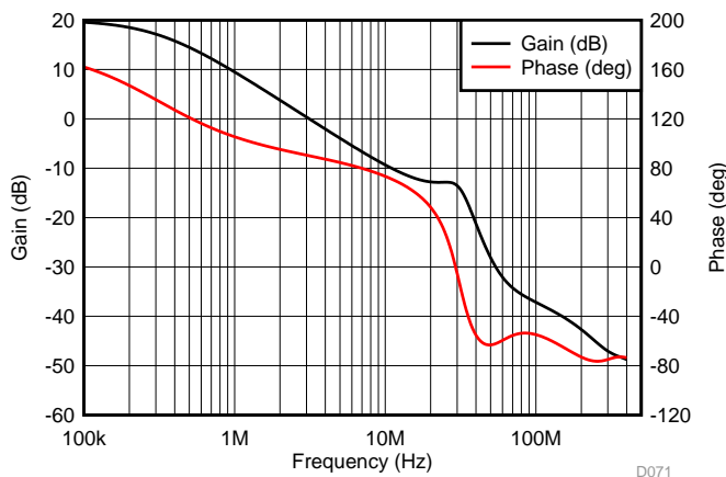
图 89. Gain and Phase Plot with a Differential Input Capacitor
