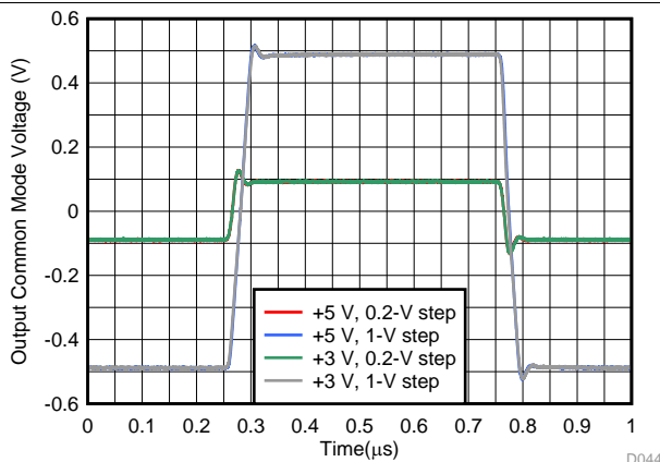
图 44. Common-Mode Voltage, Small- and Large-Step Response (VOCM Pin Driven)
