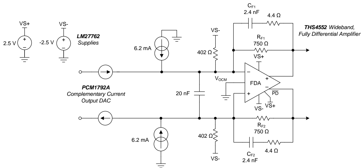
图 93. PCM1792A DAC Output Driver
