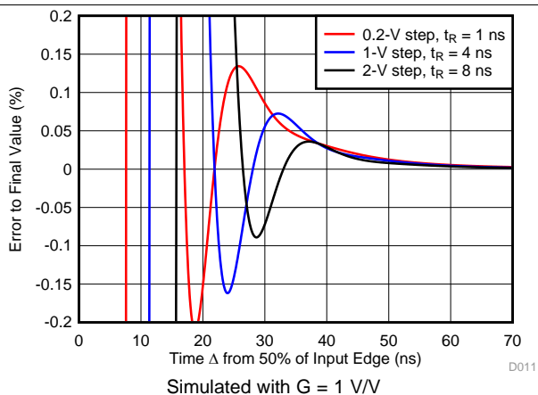
图 11. Small- and Large-Signal Step Settling Time
