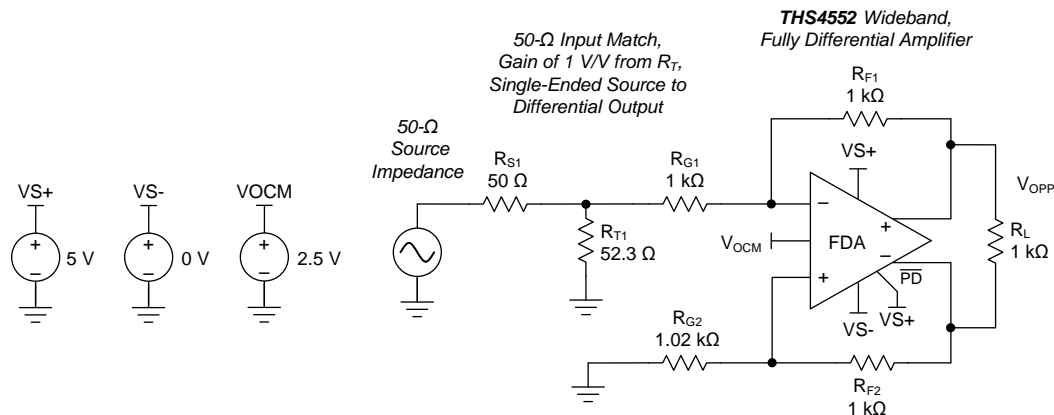
图 74. DC-Coupled Gain of 1 with R_F = 1 \text{ k}\Omega and Single-to-Differential Matched Input 50-Ω Impedance
