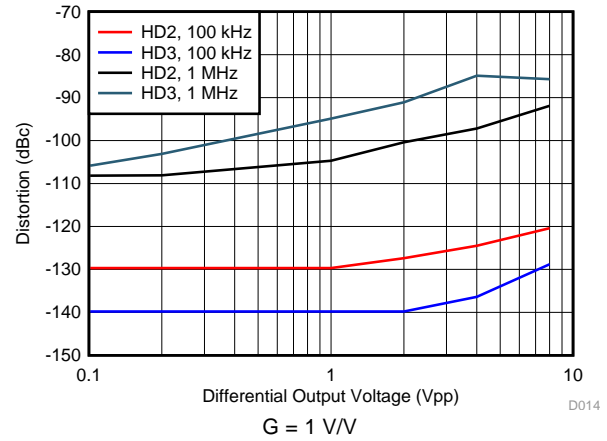
图 14. Harmonic Distortion vs Output Swing
