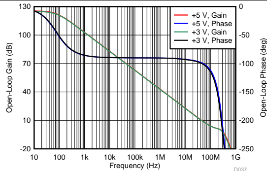
图 37. Main Amplifier Differential Open-Loop Gain and Phase vs Frequency
