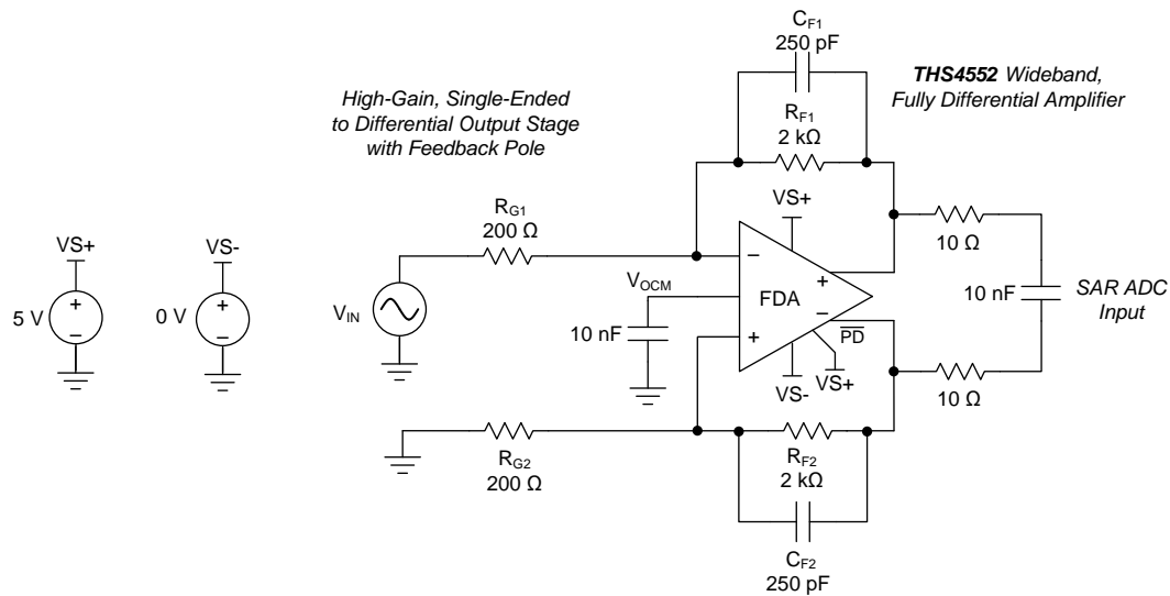
图 86. Single-Ended to Differential Stage with a Feedback Pole
