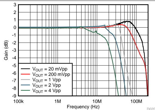
图 20. Frequency Response vs V_{OUT}
