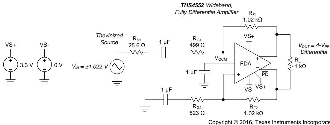
图 70. Input Swing Analysis Circuit with AC-Coupled, Single-Ended to Differential Signal Path
