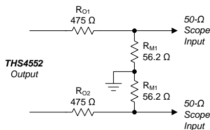
图 64. Output Interface for DC-Coupled Differential Outputs
