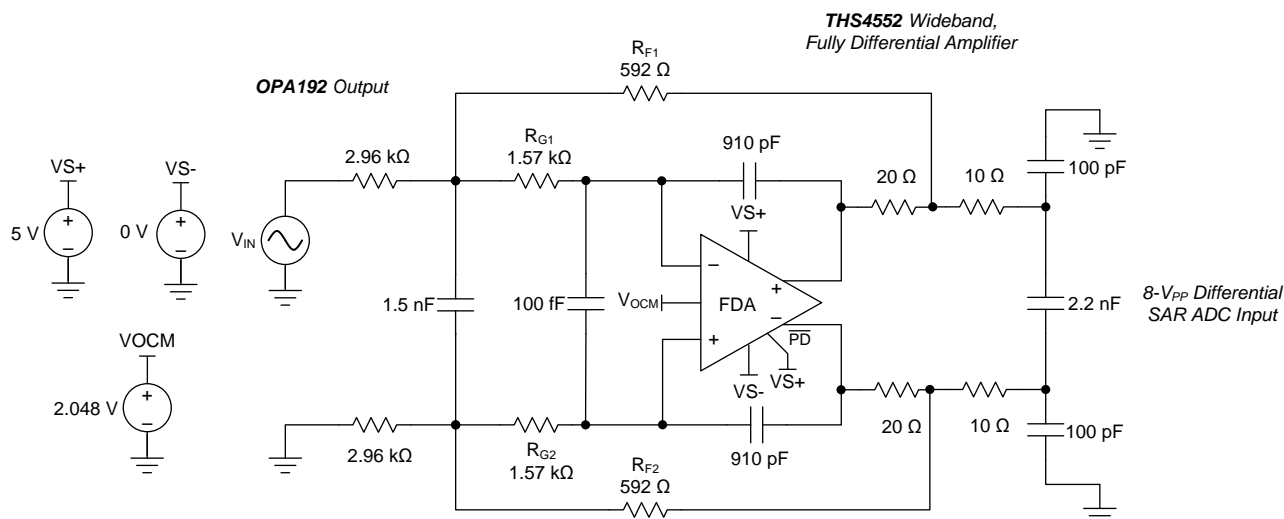
图 90. Example 100-kHz Butterworth Filter
