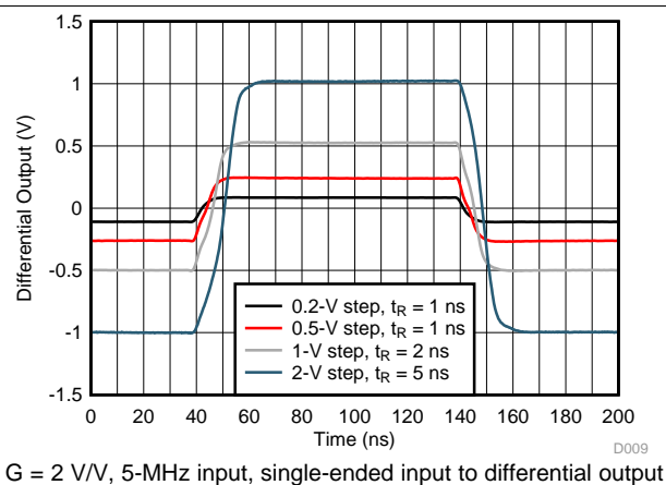
图 9. Small- and Large-Signal Step Response
