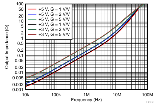
图 38. Closed-Loop Output Impedance vs Frequency
