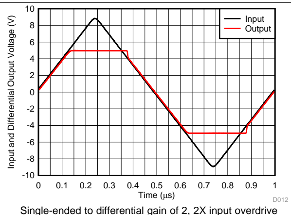
图 12. Overdrive Recovery Performance
