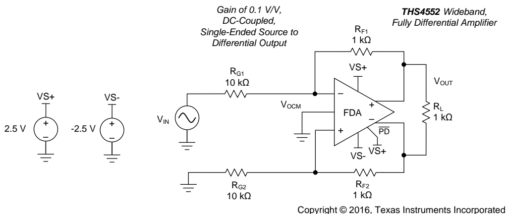
图 83. Divide-by-10 Attenuator Application for the THS4552
