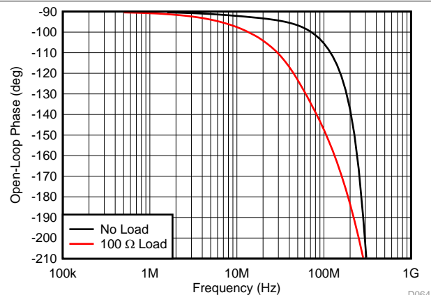
图 67. No-Load and 100-Ω A_{OL} Phase
