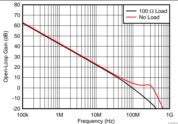
图 66. No-Load and 100-Ω Loaded A_{OL} Gain
