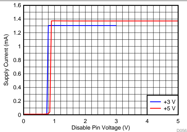
图 56. Supply Current vs \overline{\text{PD}} Voltage
