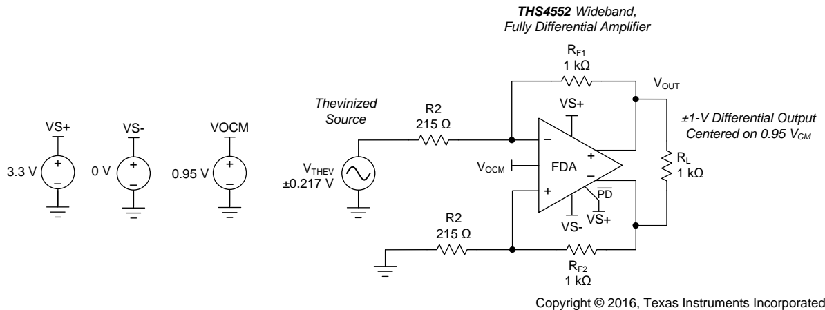
图 72. Input V_{ICM} Analysis Circuit From the Design of 图 96
