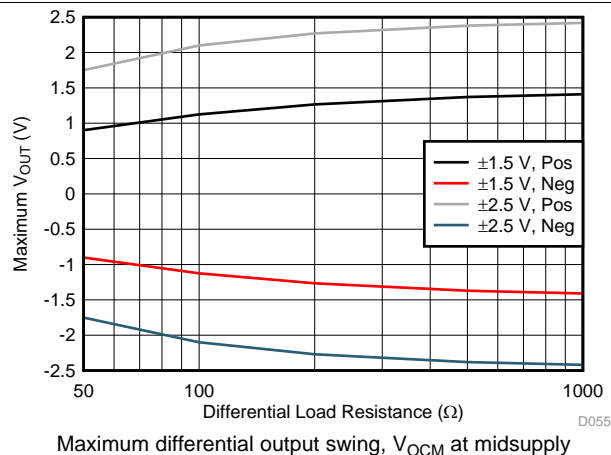
图 55. \pm Maximum V_{\text{OUT}} vs Differential Load Resistance
