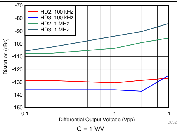
图 32. Harmonic Distortion vs Output Swing
