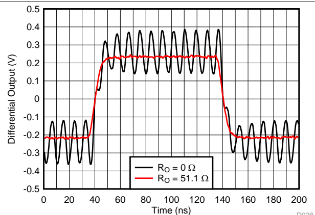
图 26. Step Response Into Capacitive Load
