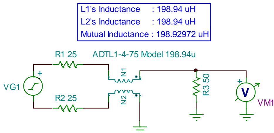
图 62. Output Measurement Balun Simulation Circuit in TINA-TI™
