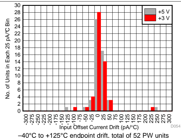
图 54. Input Offset Current Drift Histogram
