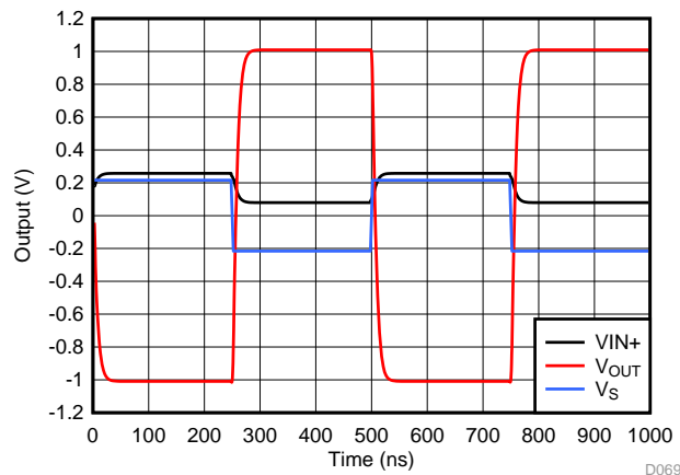
图 73. I/O Swing Simulation Using the TINA-TI™ Model
