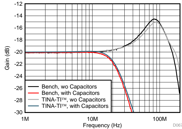
图 85. Attenuator Response Shapes With and Without External Capacitors
