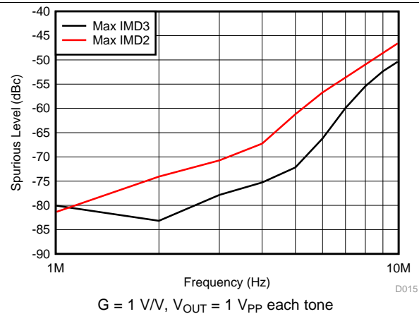
图 15. Intermodulation Distortion (IMD2 and IMD3) vs Frequency
