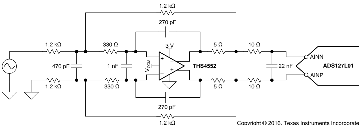
图 78. 500-kHz Low-Pass Active Filter
