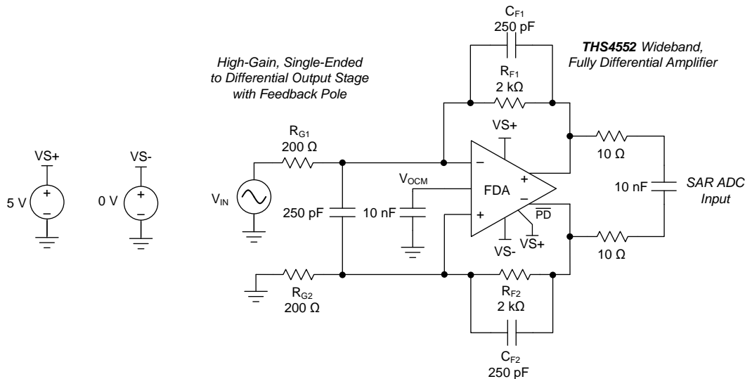
图 88. Single-Ended to Differential Stage with a Feedback Pole and Differential Input Capacitor
