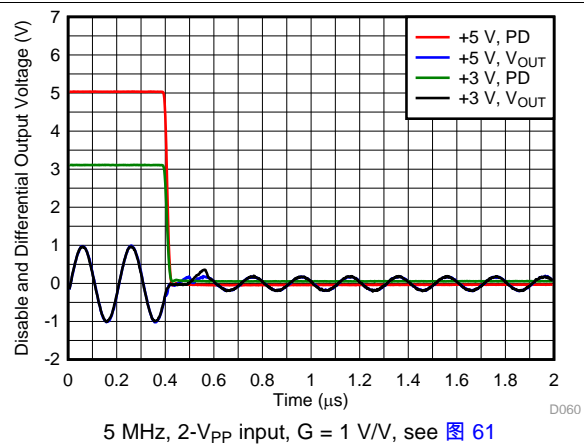
图 60. \overline{\text{PD}} Turn-Off Waveform
