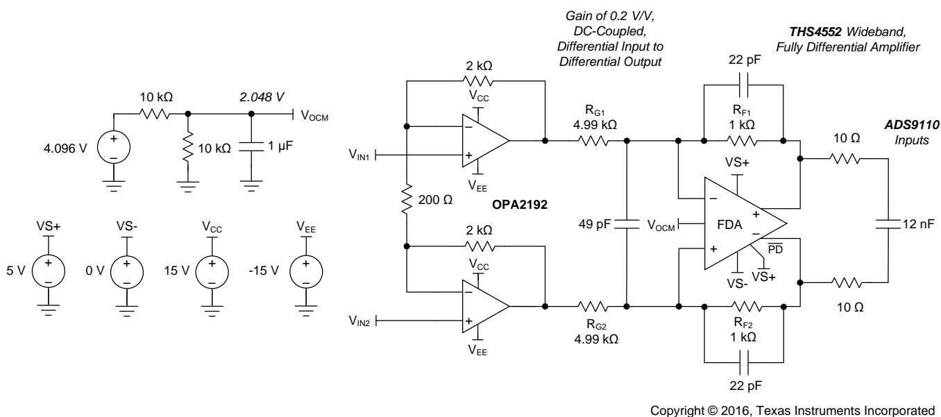
图 76. Example DC-Coupled Differential I/O Design from a Precision Dual Op Amp to an 18-Bit SAR
