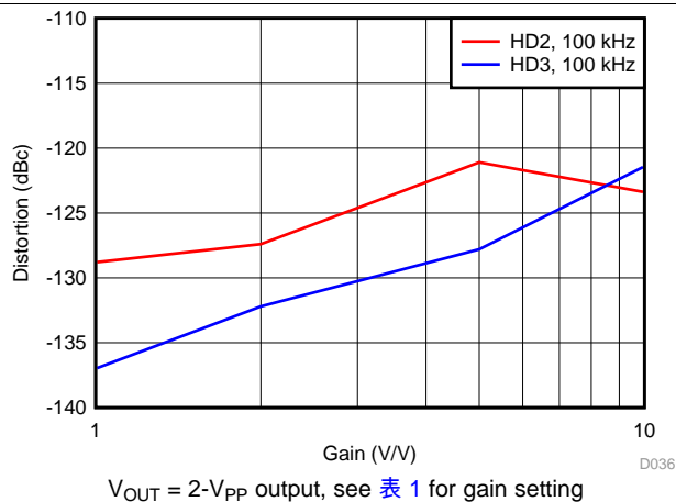
图 36. Harmonic Distortion vs Gain
