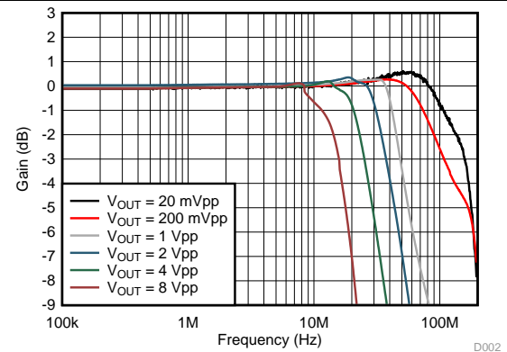
图 2. Frequency Response vs V_{OUT}
