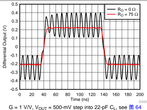
图 8. Step Response Into Capacitive Load
