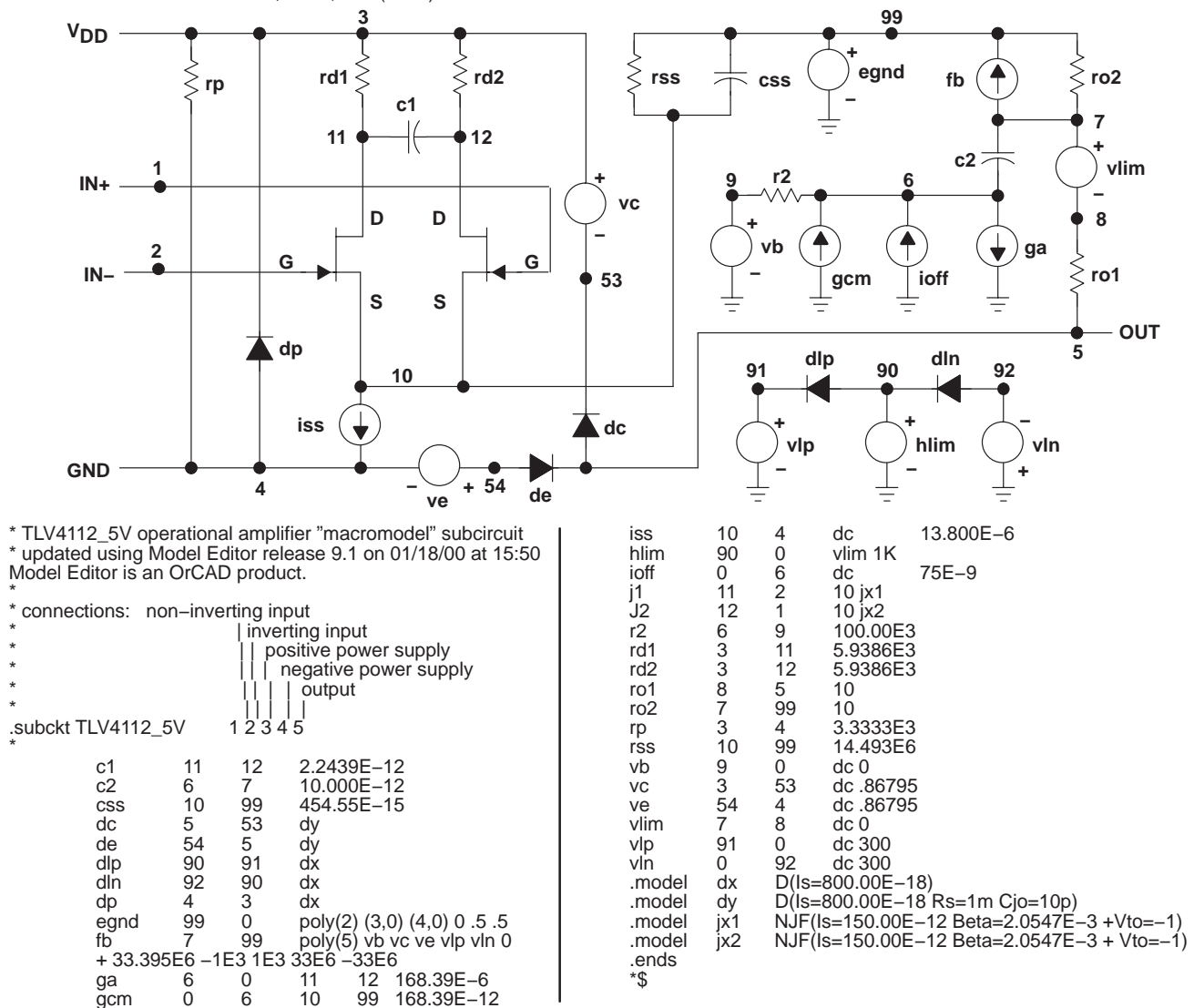
Figure 32. Boyle Macromodel and Subcircuit
