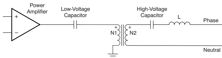
Figure 27. Simplified Line-Coupling Circuit
