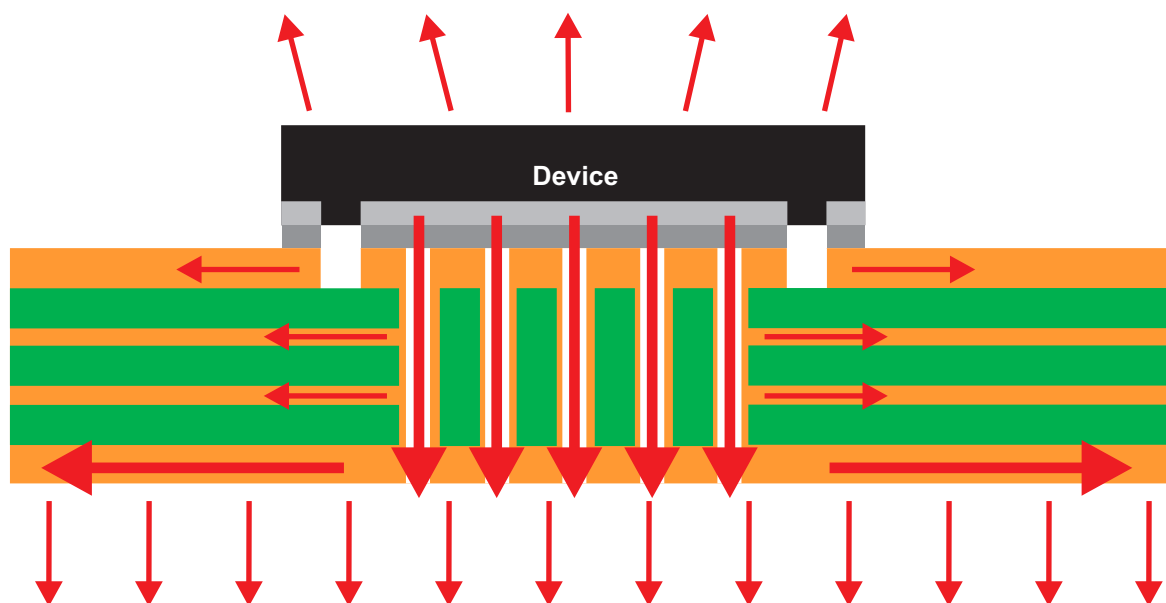
Figure 31. Heat Spreading to PCB
