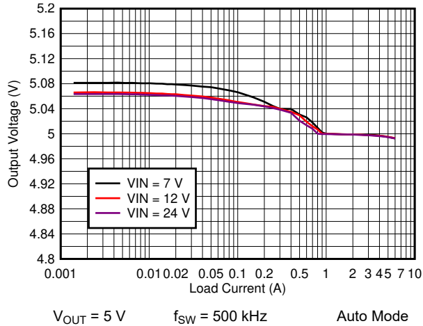
Figure 8-9. TPS7H4010-SEP Load and Line Regulation
