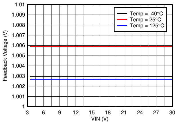
Figure 6-3. Feedback Voltage
