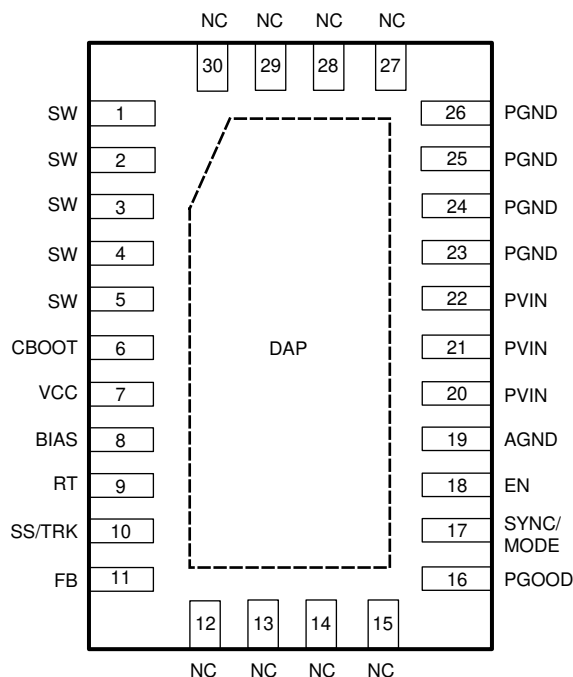
Figure 5-1. RNP Package 30-Pin QFN 6 mm × 4 mm × 0.8 mm Top View
