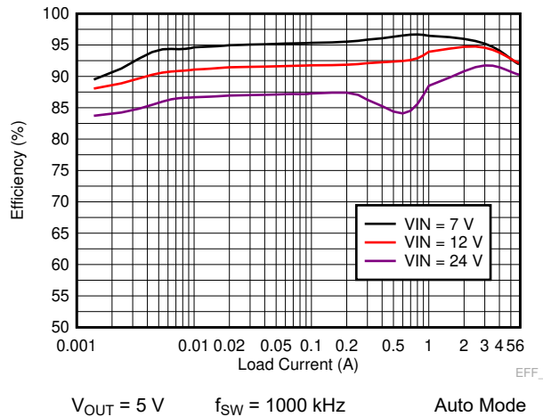
Figure 8-5. TPS7H4010-SEP Efficiency
