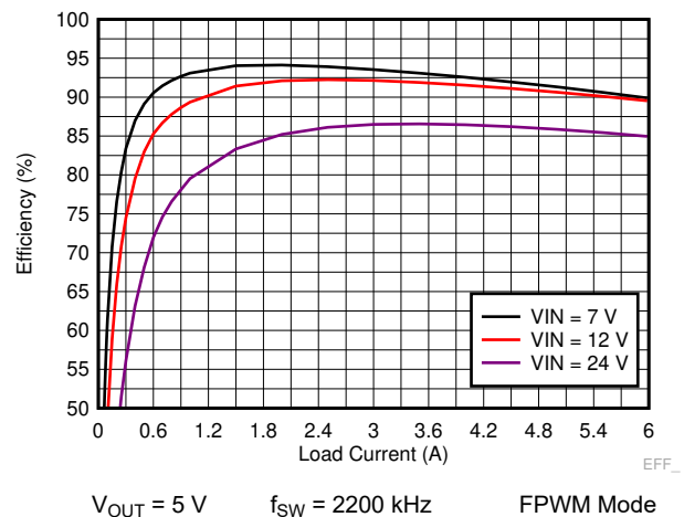
Figure 8-8. TPS7H4010-SEP Efficiency
