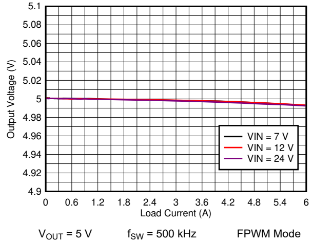
Figure 8-10. TPS7H4010-SEP Load and Line Regulation
