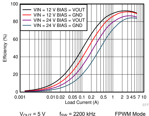
Figure 7-7. TPS7H4010 Efficiency Comparison With Bias = V_{OUT} to Bias = GND in FPWM Mode
