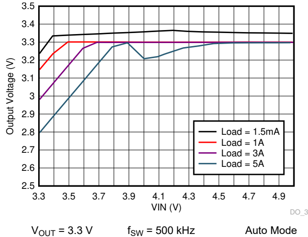
Figure 8-15. TPS7H4010-SEP Dropout Curve
