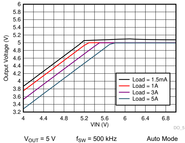
Figure 8-13. TPS7H4010-SEP Dropout Curve
