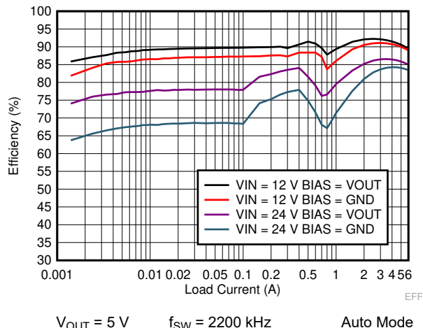
Figure 7-6. TPS7H4010 Efficiency Comparison With Bias = V_{OUT} to Bias = GND in Auto Mode
