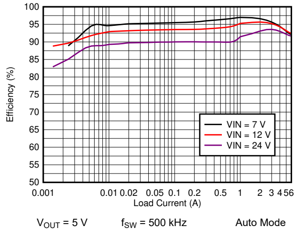
Figure 8-3. TPS7H4010-SEP Efficiency
