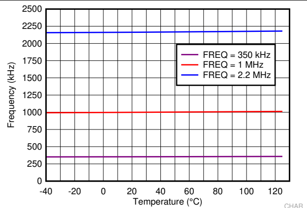
Figure 6-6. Switching Frequency Set by R_T Resistor
