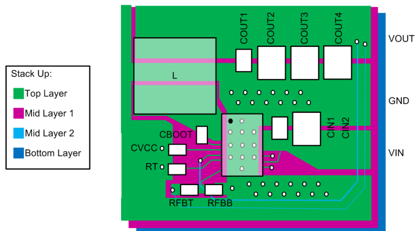
Figure 10-3. TPS7H4010-SEP Layout Example
