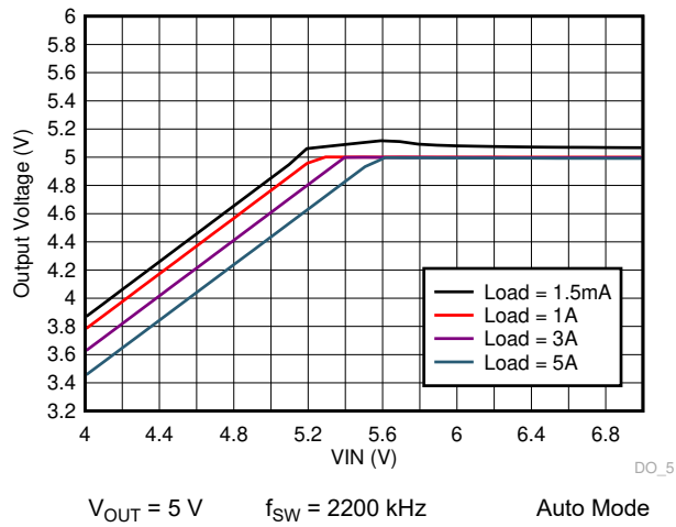
Figure 8-11. TPS7H4010-SEP Dropout Curve
