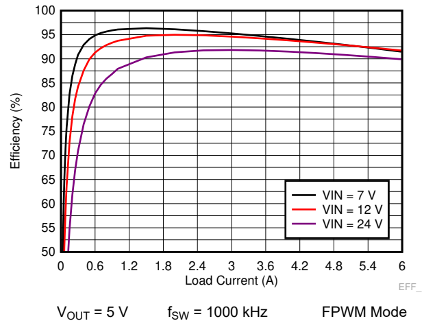
Figure 8-6. TPS7H4010-SEP Efficiency
