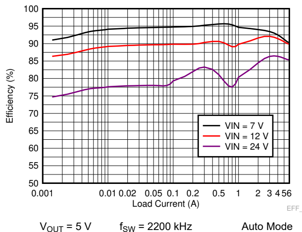
Figure 8-7. TPS7H4010-SEP Efficiency
