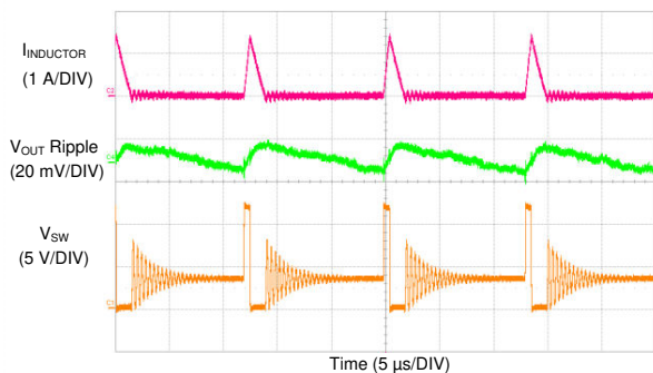
Figure 8-17. TPS7H4010-SEP Switching Waveform and V_{OUT} Ripple
