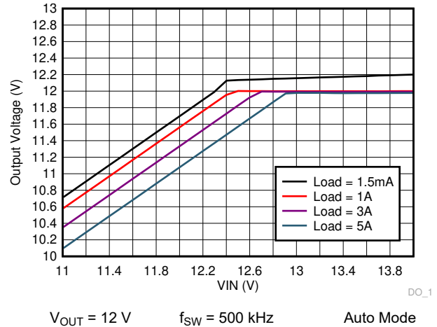
Figure 8-16. TPS7H4010-SEP Dropout Curve
