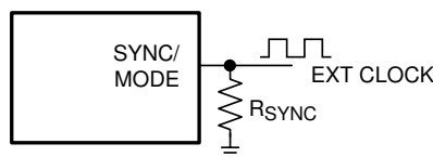
Figure 7-13. Frequency Synchronization
