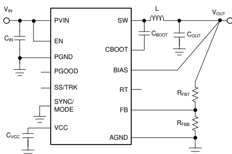
Simplified Schematic
