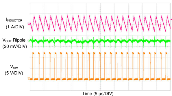
Figure 8-18. TPS7H4010-SEP Switching Waveform and V_{OUT} Ripple
