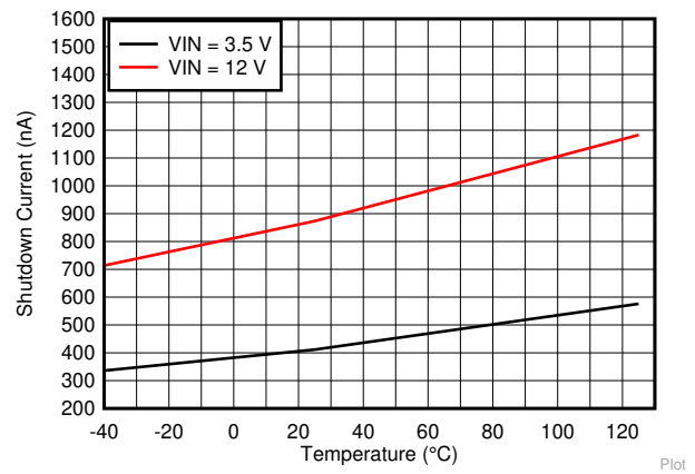
Figure 6-2. Shutdown Quiescent Current
