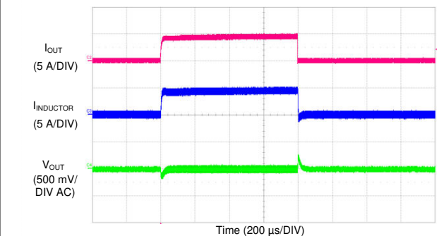
Figure 8-30. TPS7H4010-SEP Load Transients
