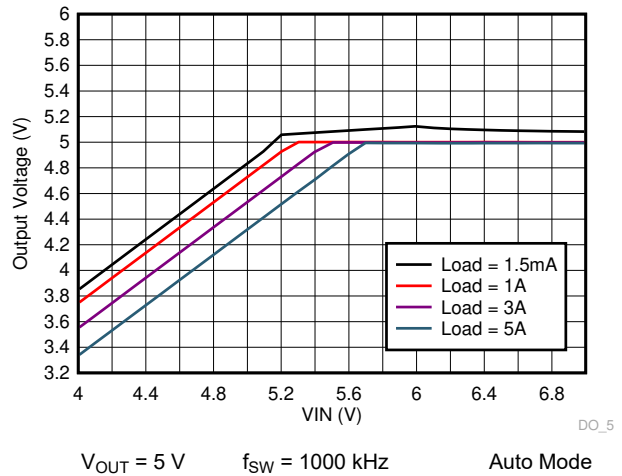
Figure 8-14. TPS7H4010-SEP Dropout Curve
