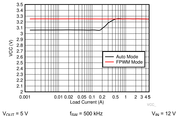
Figure 7-8. VCC Voltage vs Load Current
