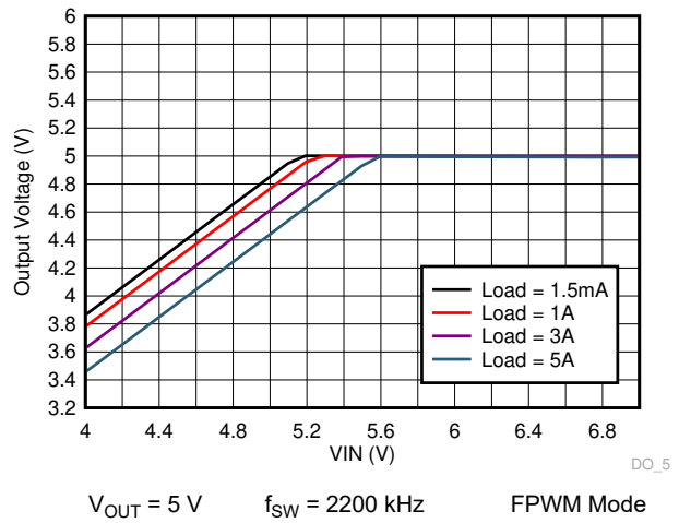
Figure 8-12. TPS7H4010-SEP Dropout Curve
