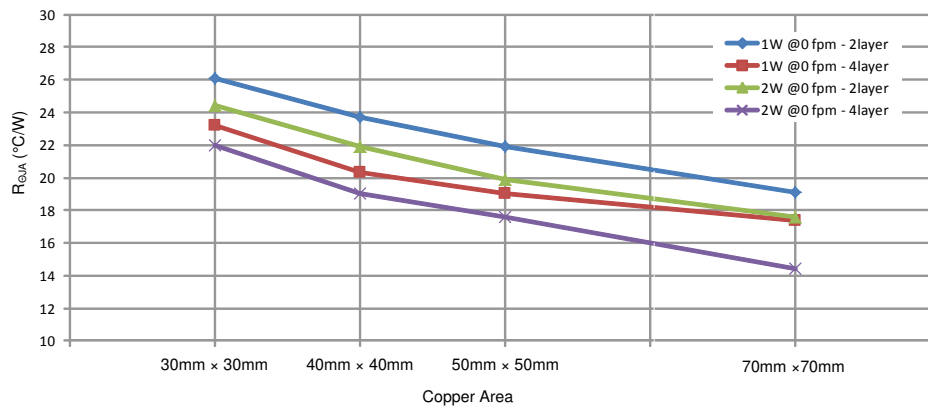
Figure 10-2. Measured R_{\theta JA} vs PCB Copper Area on 2-Layer Boards and 4-Layer Boards
