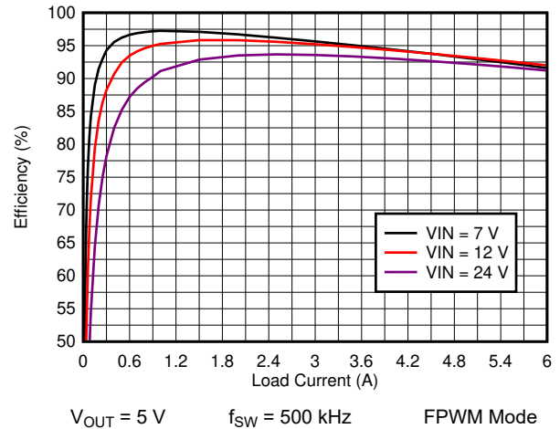
Figure 8-4. TPS7H4010-SEP Efficiency
