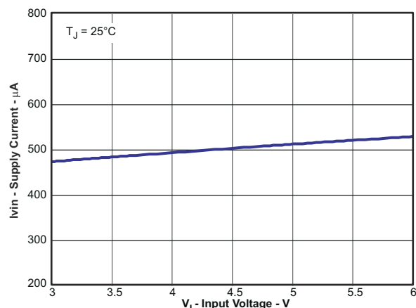
Figure 6-17. Supply Current vs Input Voltage
