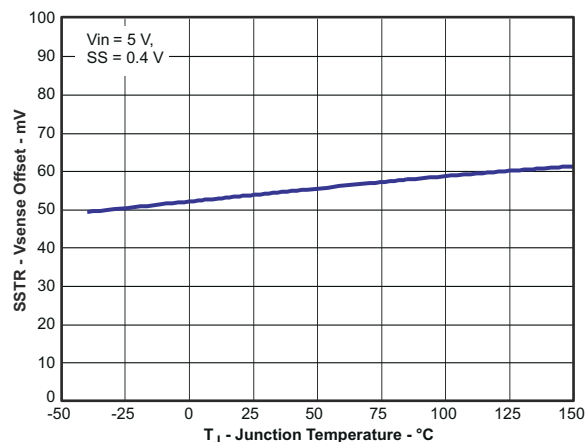
Figure 6-20. SS/TR to VSENSE Offset vs Junction Temperature
