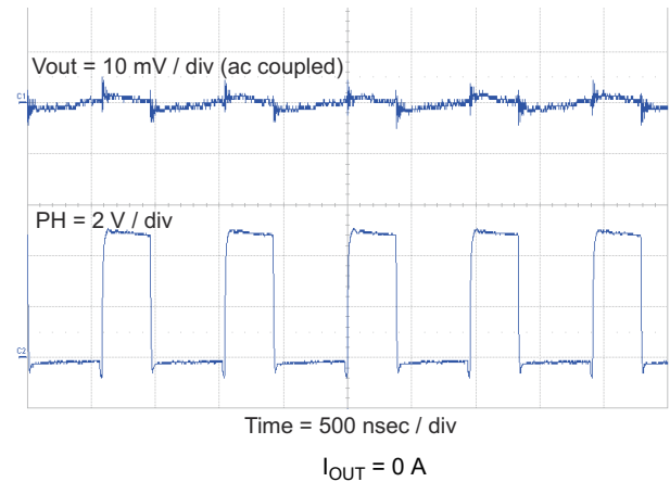
Figure 8-7. Output Ripple
