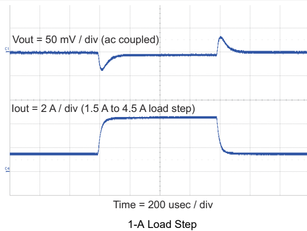
Figure 8-4. Transient Response
