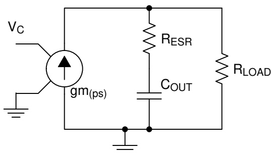
Figure 7-12. Small Signal Model for Peak Current Mode Control
