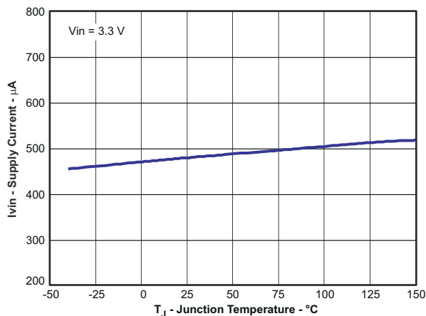
Figure 6-16. Supply Current vs Junction Temperature
