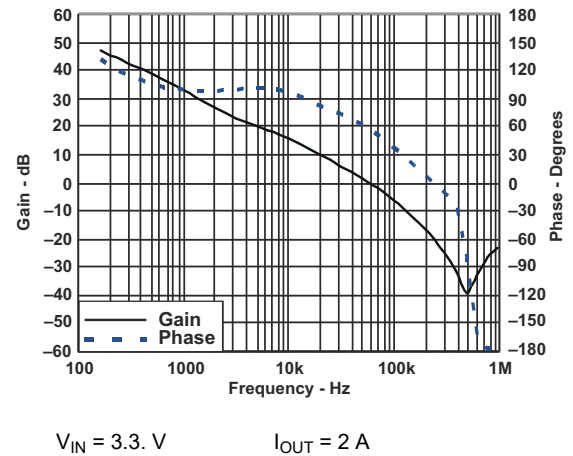
Figure 8-9. Closed-Loop Response
