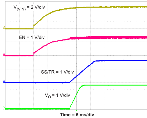
图 39. Power-Up V_O , V_{(VIN)}
