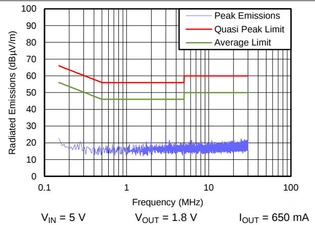
Figure 8. Conducted EMI Default Evaluation Board BOM With Additional 2.2μH 1μF LC Input Filter
